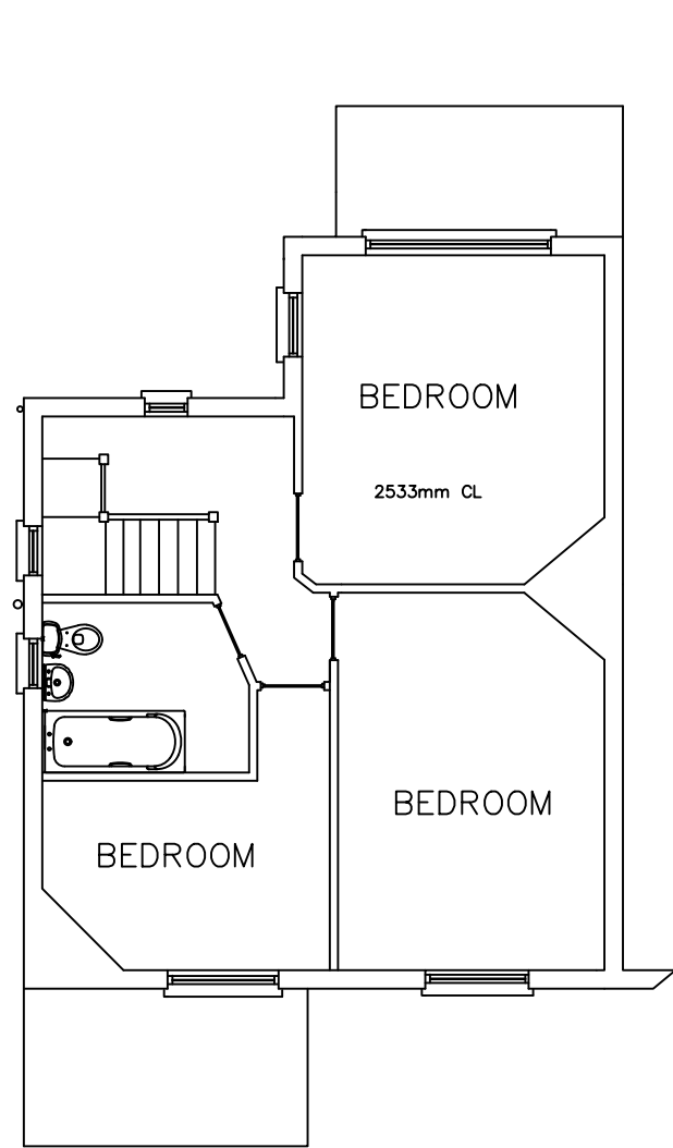
PROPOSED FIRST FLOOR LAYOUT
