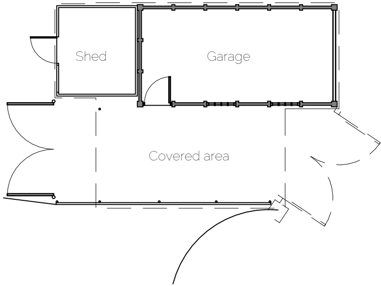
Existing Floor Plan 1:100
