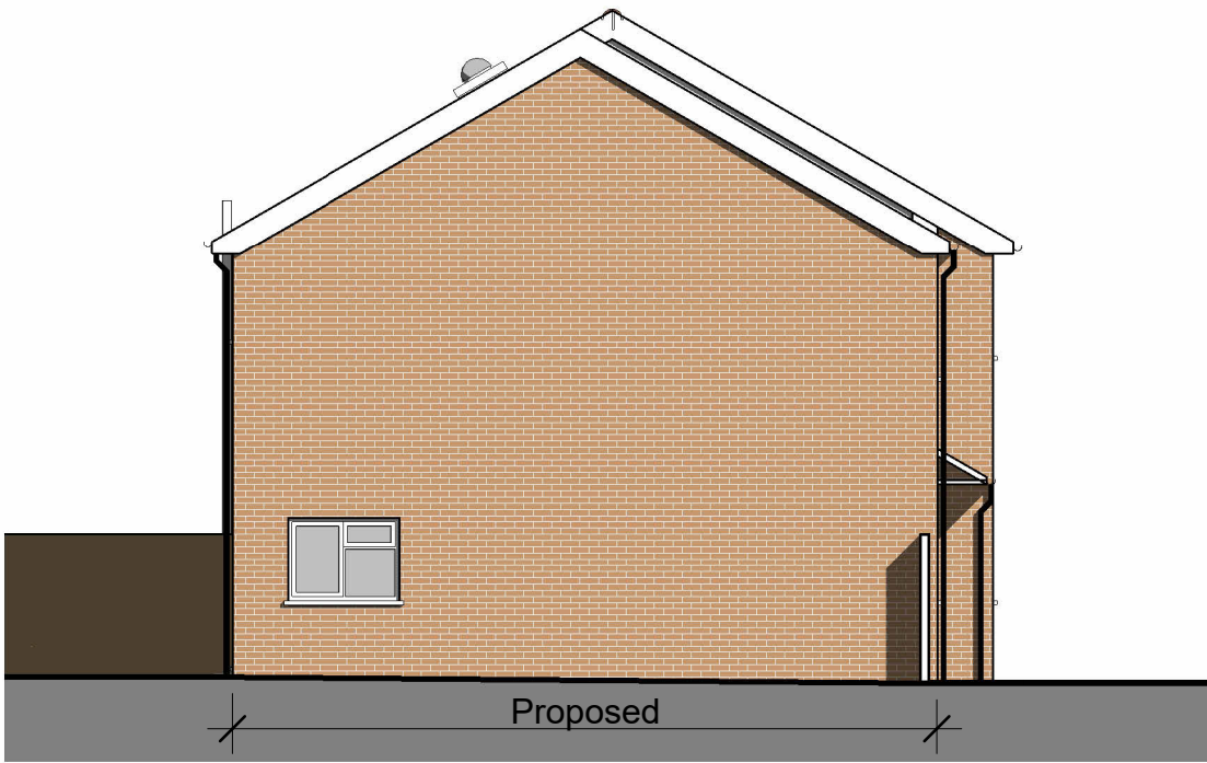
Proposed Side (West) Elevation 1 : 100
