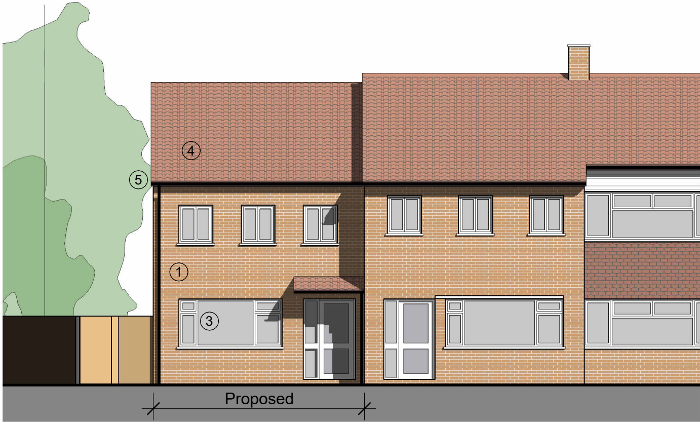
Proposed Front (South) Elevation 1 : 100
