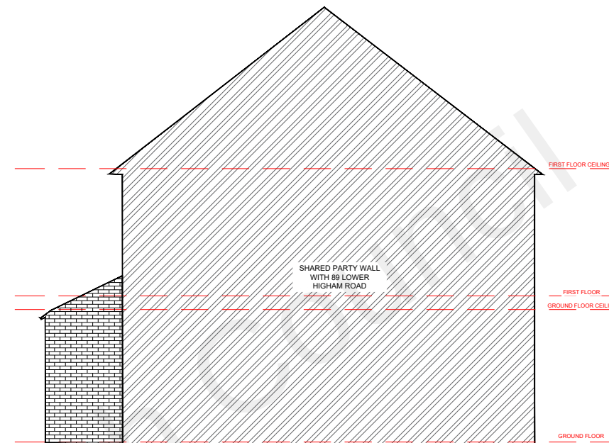
ELEVATION REFERENCE D-D
