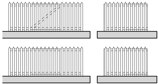
Proposed 1.5m timber fence elevations (refuse enclosure) 1:100 @ A3
