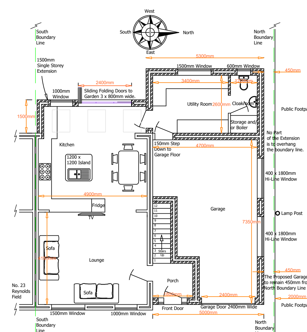
Proposed Ground Floor Plan "L" 1:100
