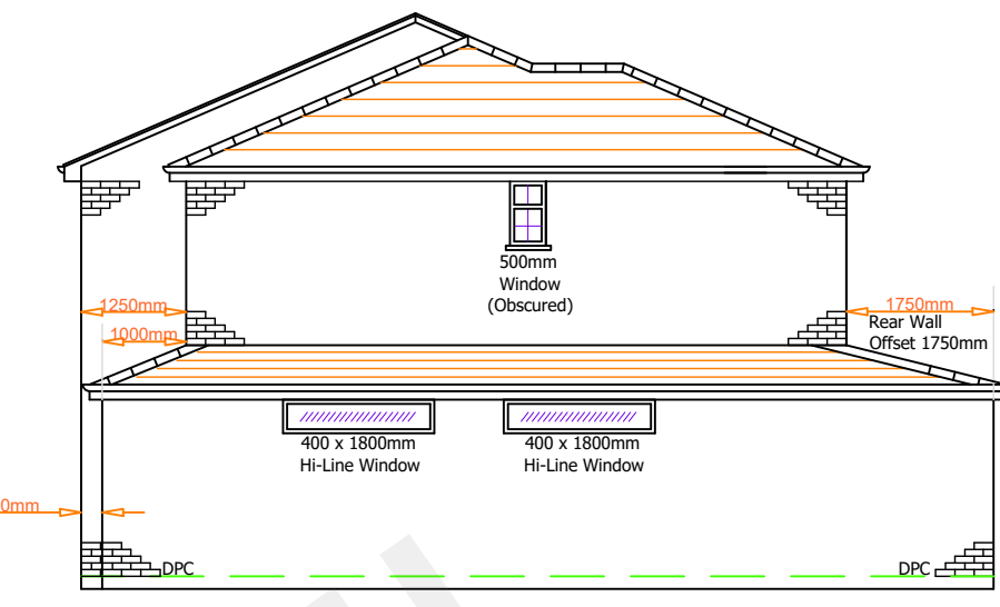
Proposed Side (North) Elevation 1:100
