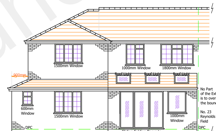
Proposed Rear (West) Elevation 1:100
