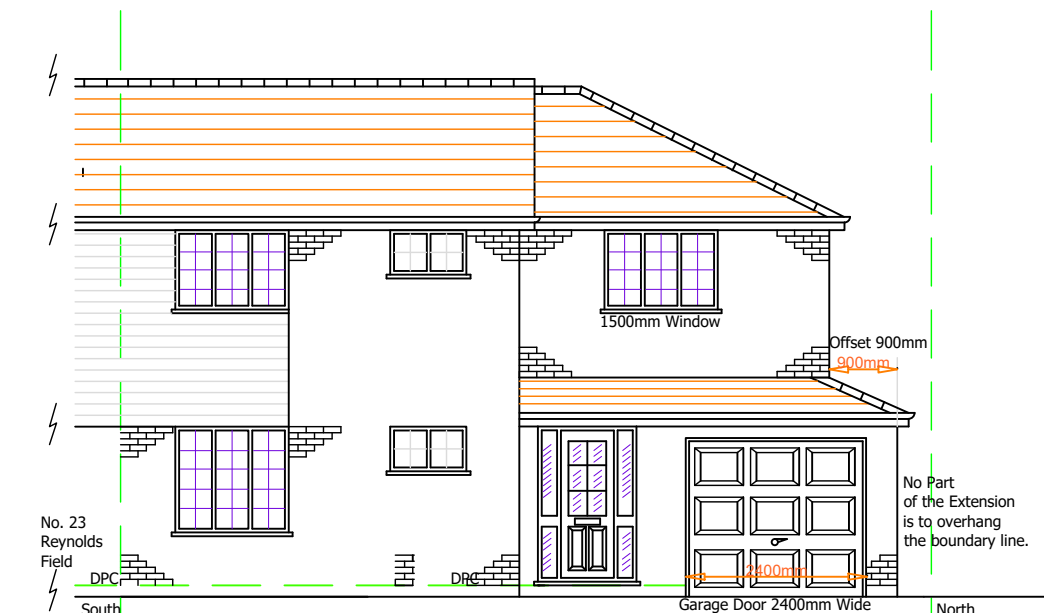
Proposed Front (East) Elevation Plan 1:100
