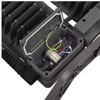
Electrical Connection box of BVP518 floodlight with cable gland and push-in terminals enabling electrical connection to driver box (Grey painted housing)
