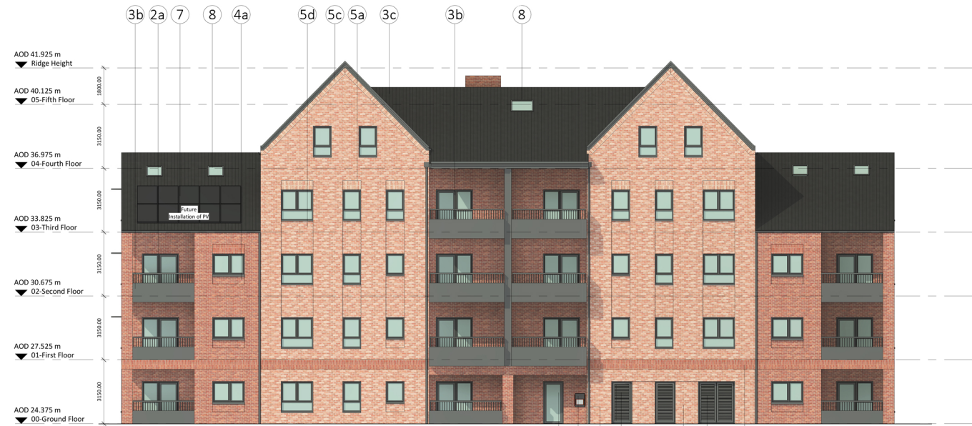
Block A - East Elevation
