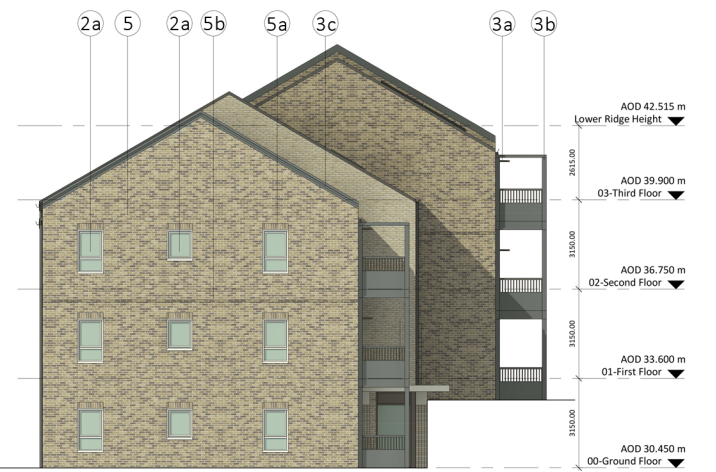
Block B - West Elevation
