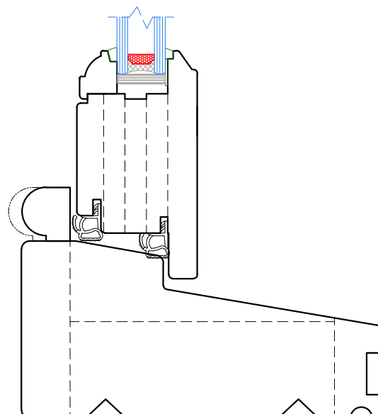
INTEGRATED VERTICAL SLIDER'S CILL WITH REBATE FOR CILL EXTENSION
