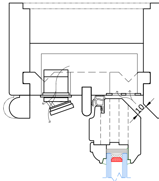
VERTICAL SLIDER WITH HIDDEN TRICKLE VENT
