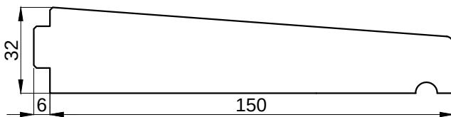
ALL AVAILABLE SIZES OF CILLS EXTENSIONS 1:2
