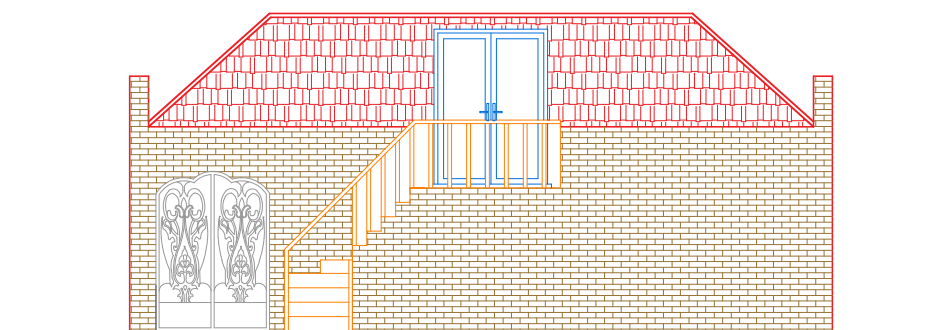
PROPOSED REAR ELEVATION OF GARAGE
