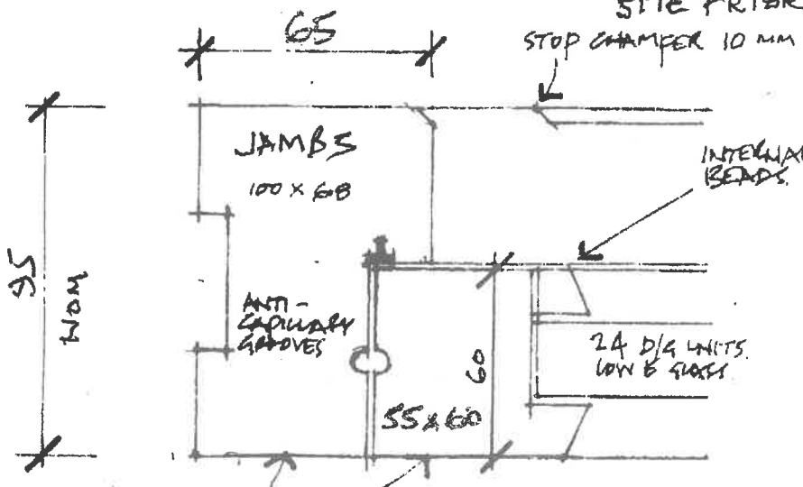
PLAN: WINDOW JAMBS
