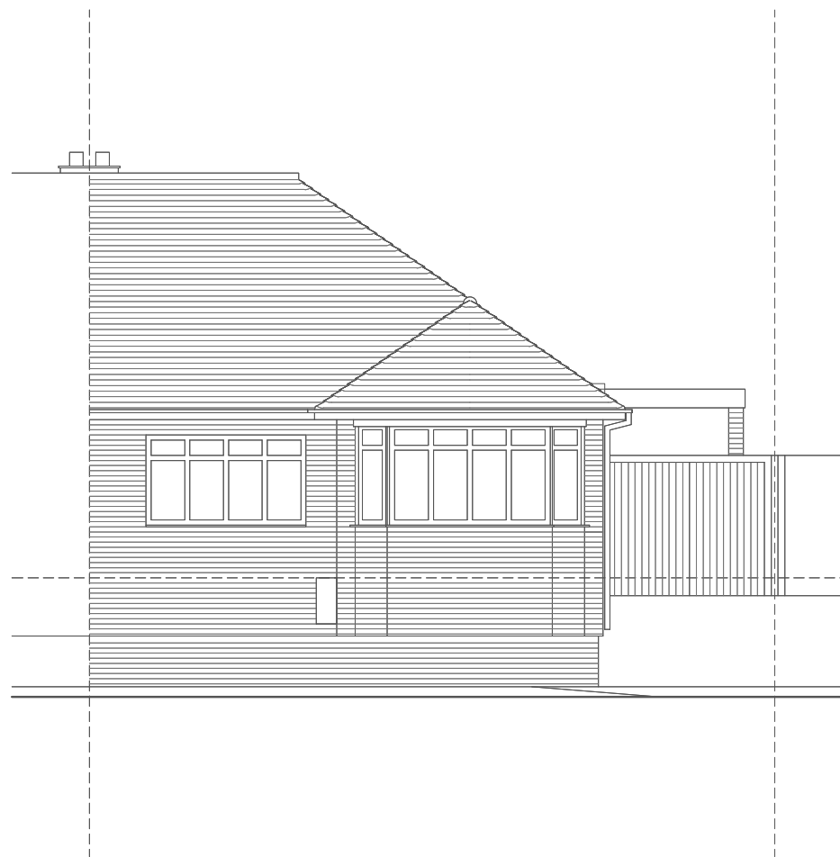
South West Elevation
