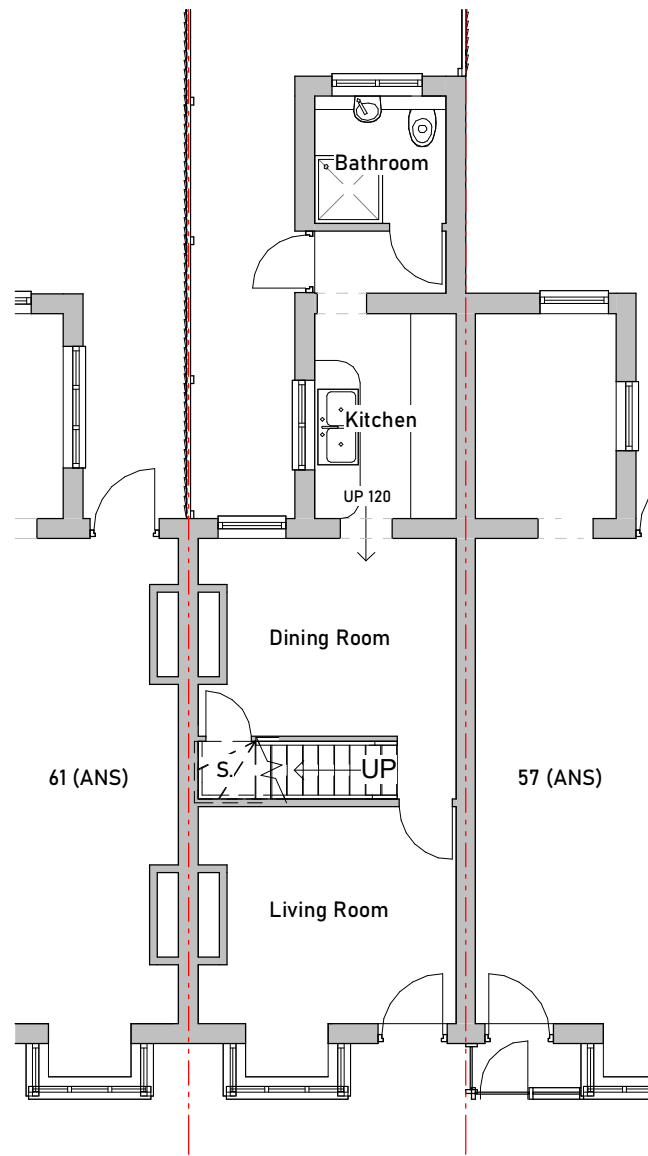
01 - Ground Floor 1 : 100
