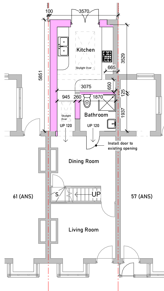
01 - Ground Floor 1 : 100
