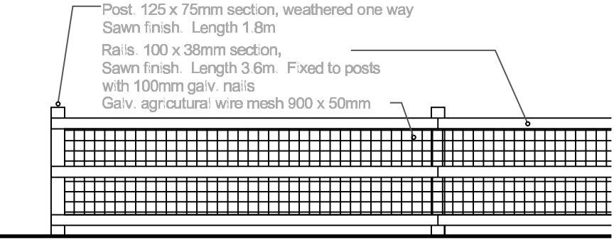
Post and Rail Fence Elevation 1:50
