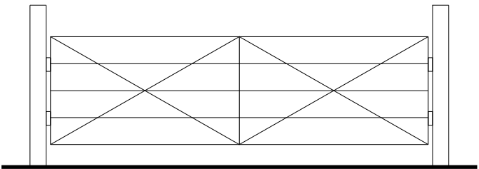
Timber Field Gate Elevation 1:50
