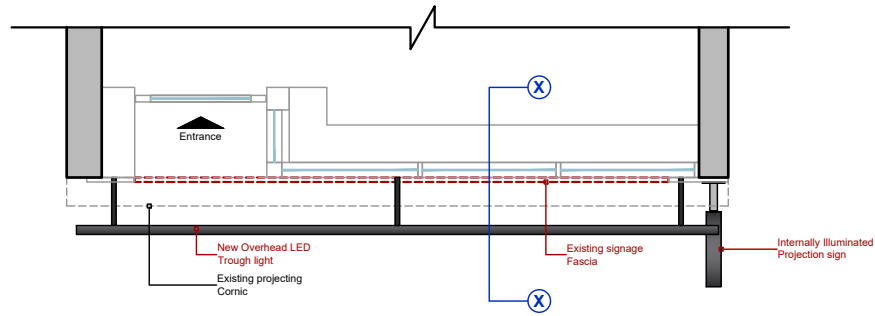
A Proposed Plan Scale 1:50 @ A3
