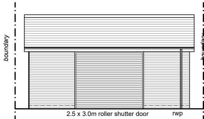
REAR ELEVATION (1:100)
