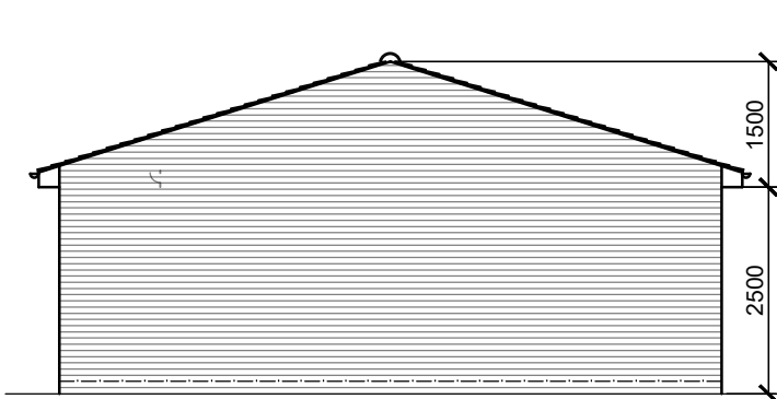
SIDE ELEVATION (1:100)
