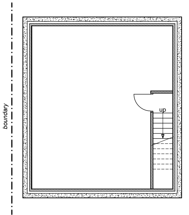
BASEMENT FLOOR PLAN (1:100)
