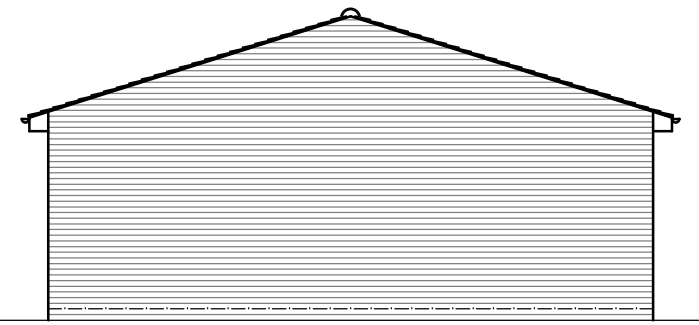
SIDE ELEVATION (1:100)
