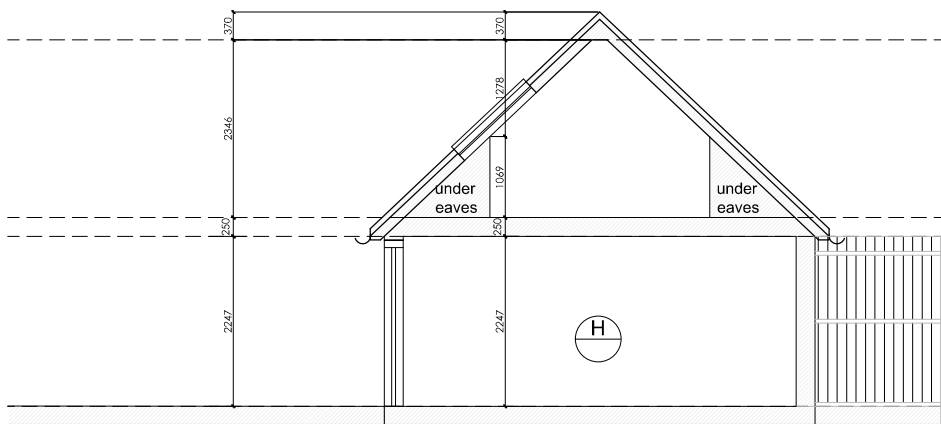
Existing Section B-B
