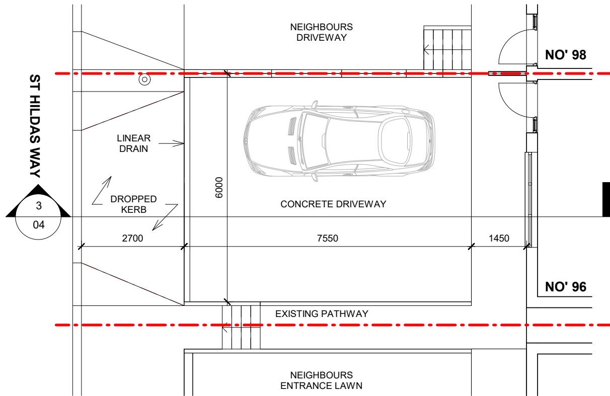
1 PROPOSED GROUND FLOOR PLAN
