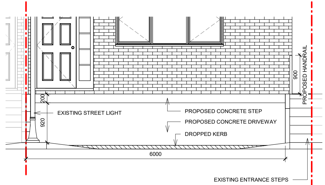
2 FRONT ELEVATION
