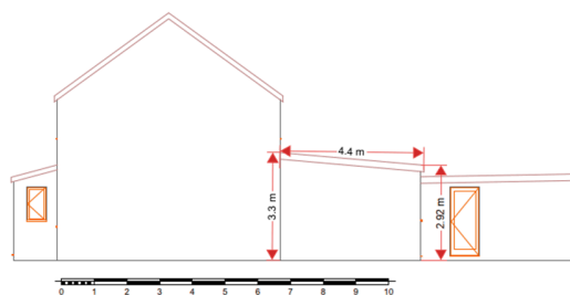
East Elevation Proposed
