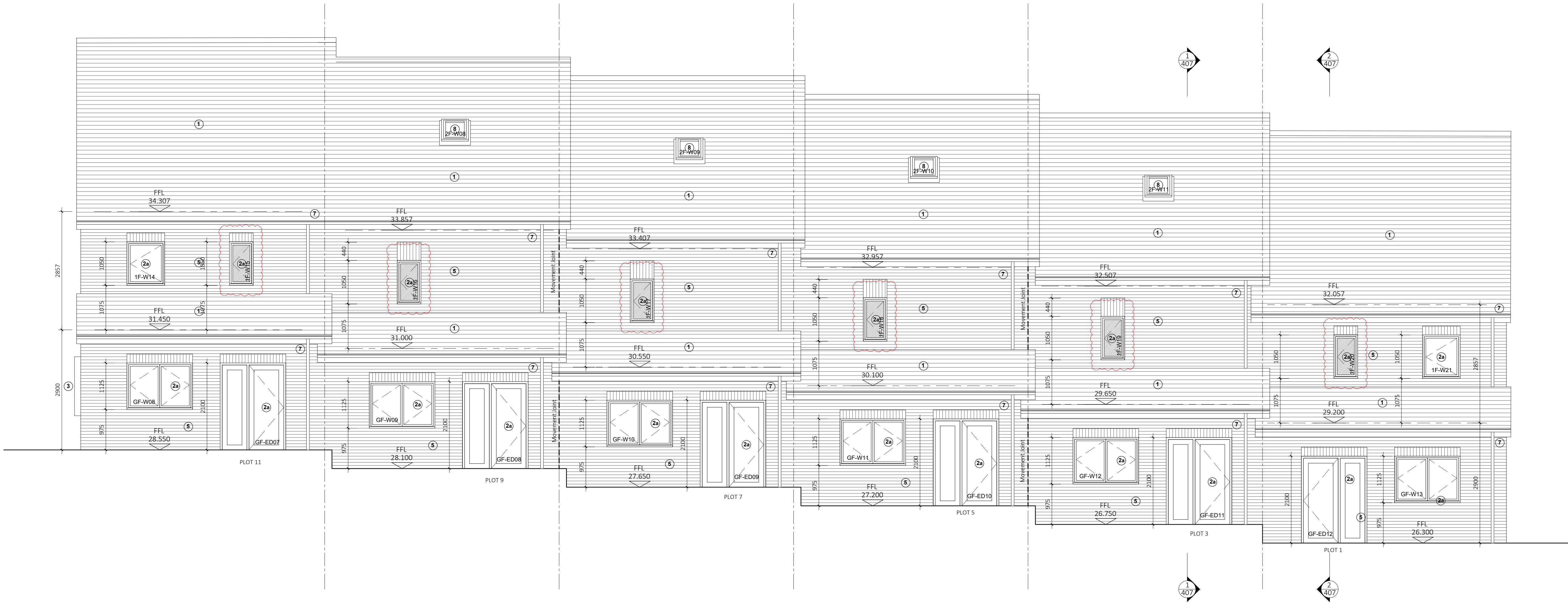
Terrace T01 - Elevations - North Scale 1:50 @ A1
