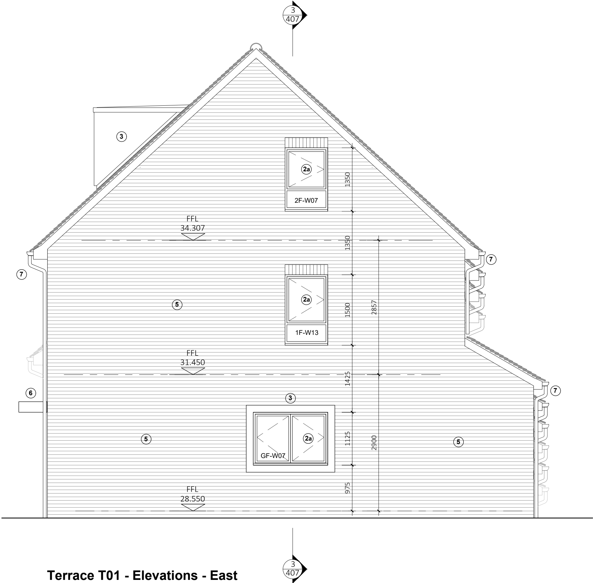
Terrace T01 - Elevations - East Scale 1:50 @ A1
