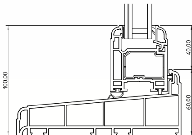
Bottom Rail
