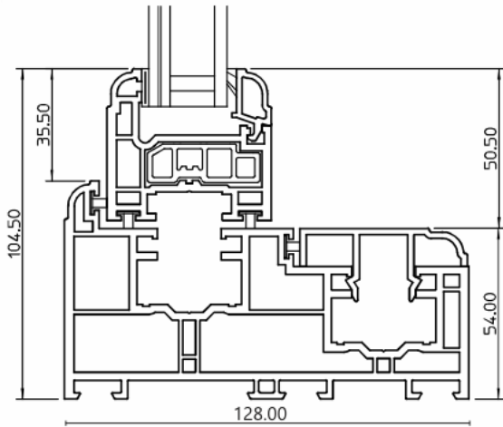
Top Rail
