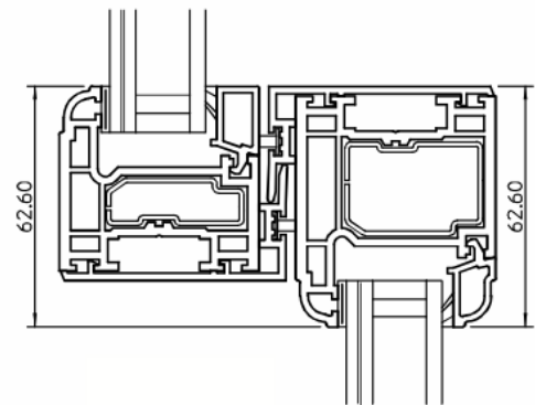
Meeting Rail
