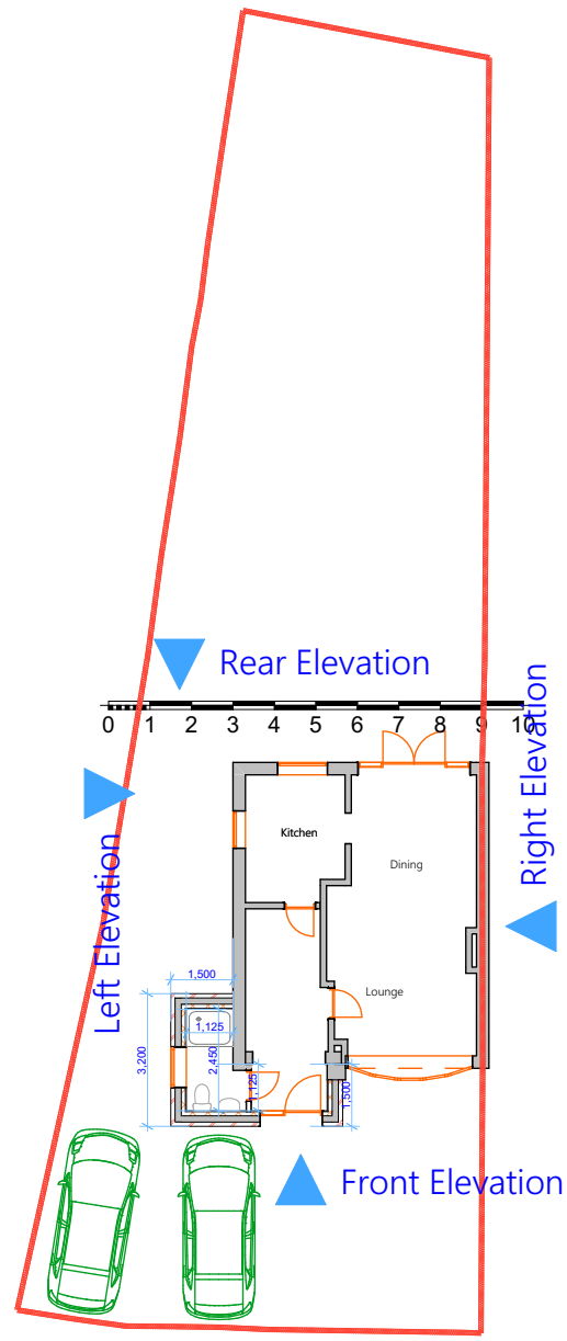
3 Site Plan Proposed 1:200
