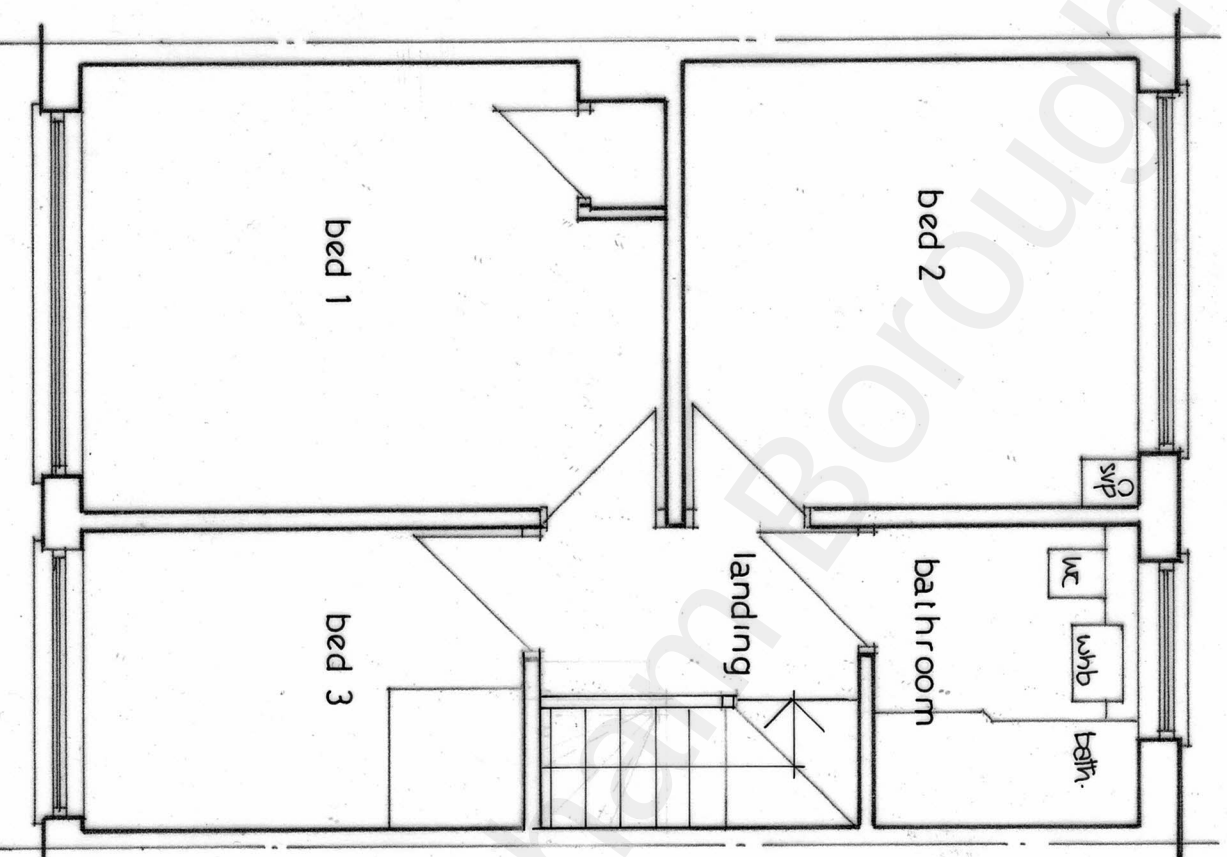
EXISTING FIRST FLOOR PLAN 1:50
