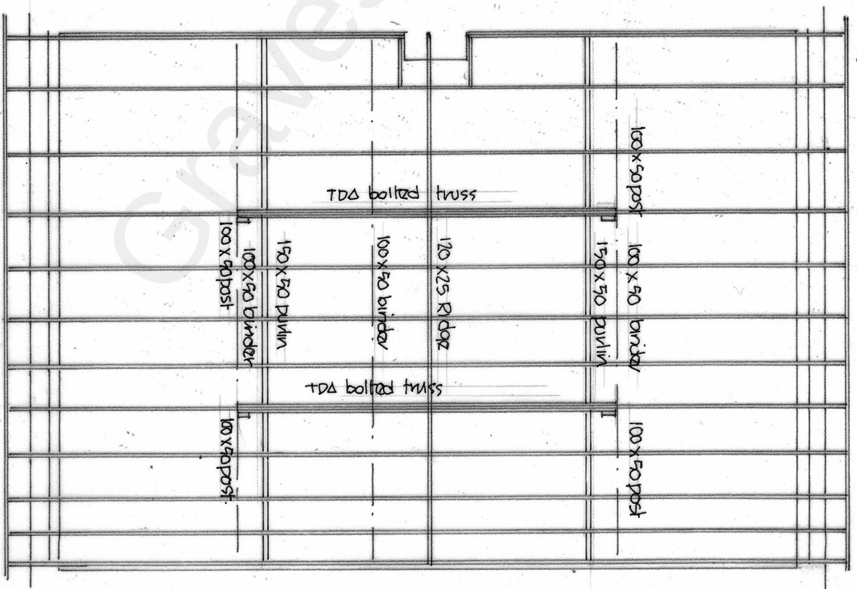
EXISTING ROOF LAYOUT 1:50
