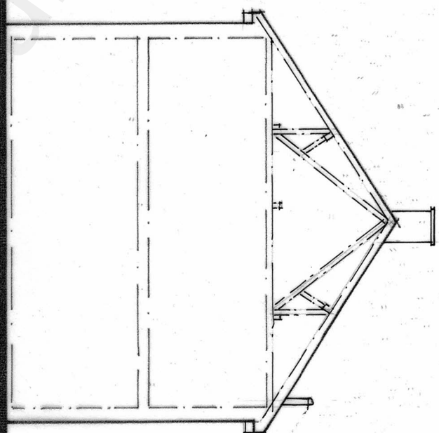
EXISTING SECTION 1:100 south
