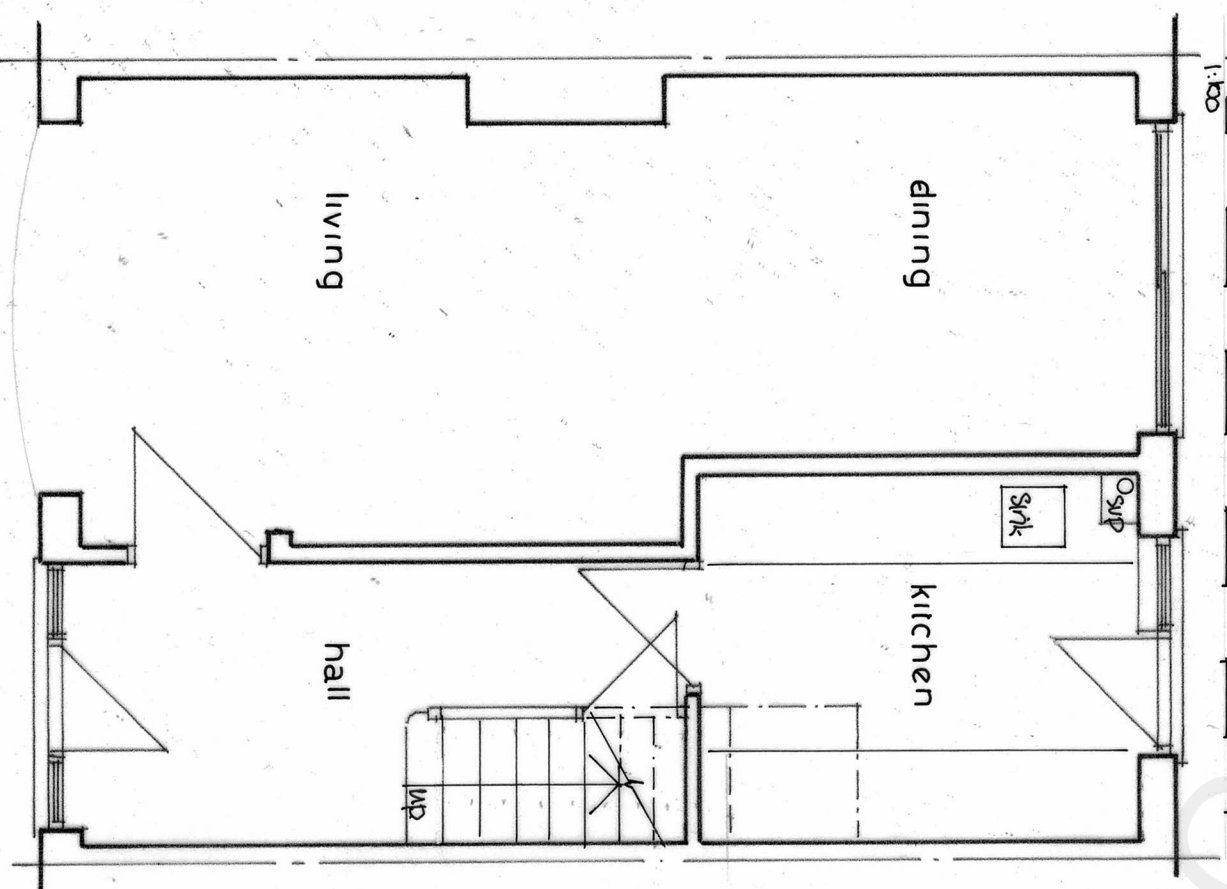
EXISTING GROUND FLOOR PLAN 1:50
