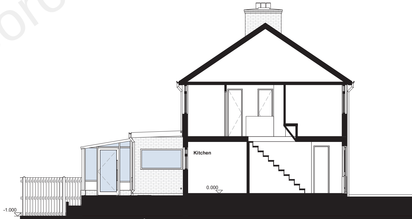
Existing Section
