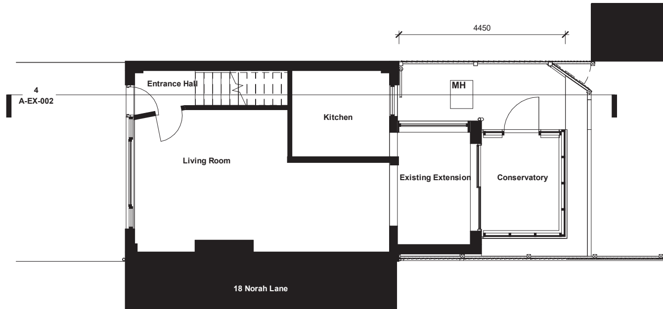
Existing Level 0
