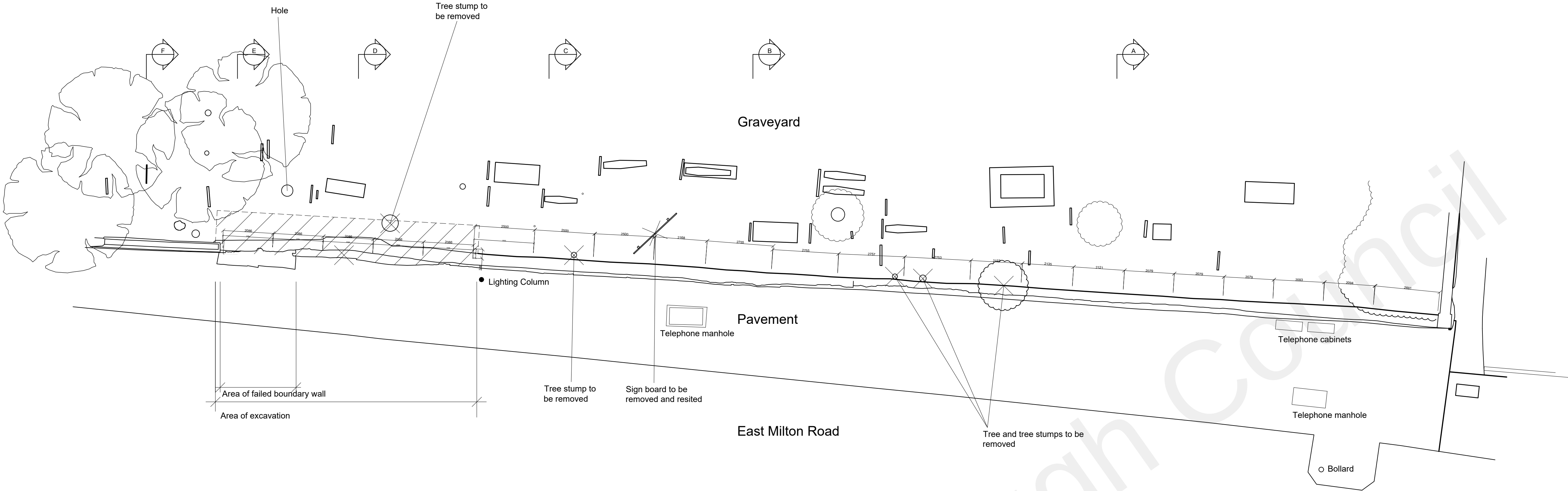
1 Existing Plan 201 1:100
