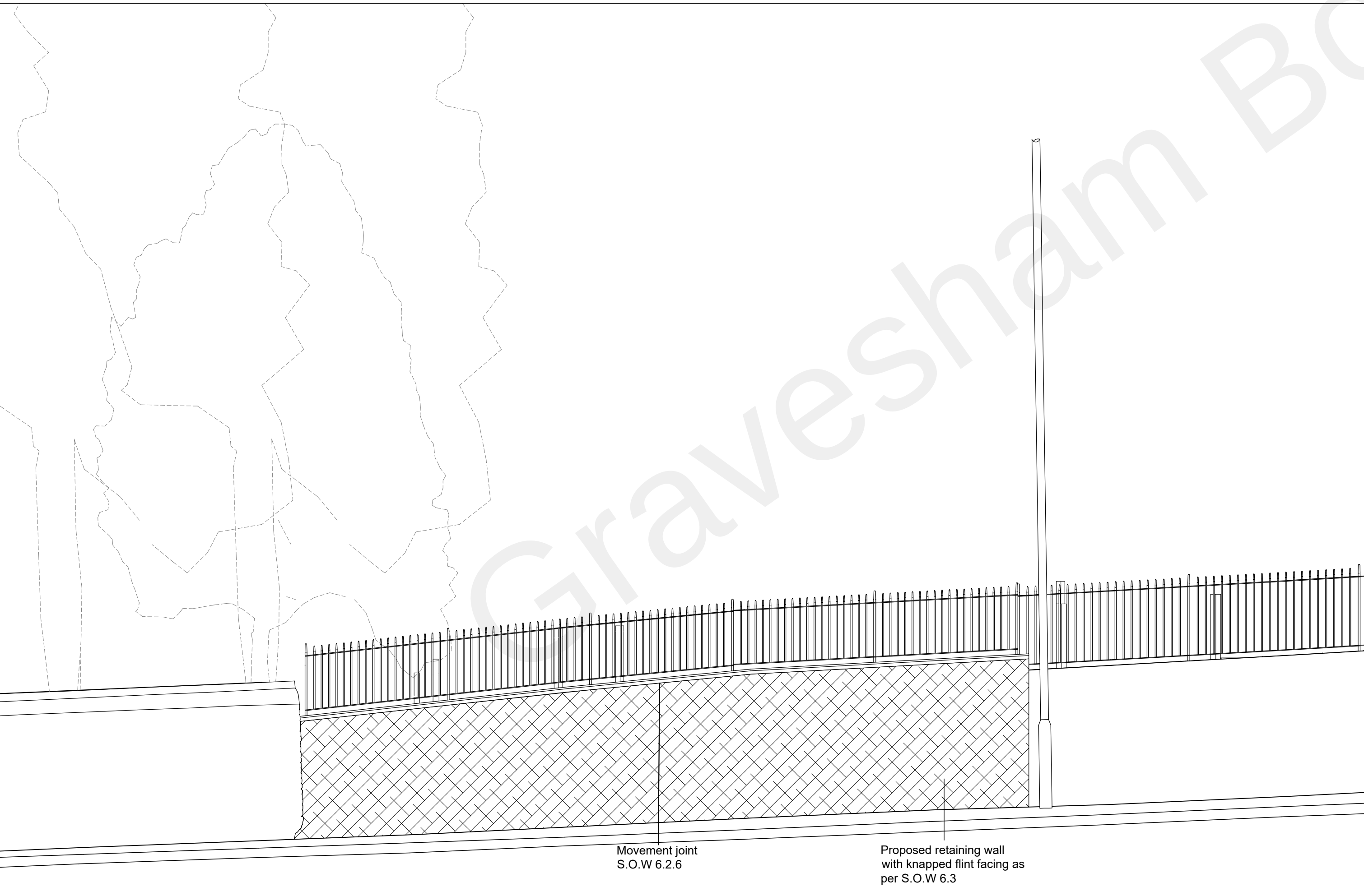
2 Proposed Elevation 214 1:50
