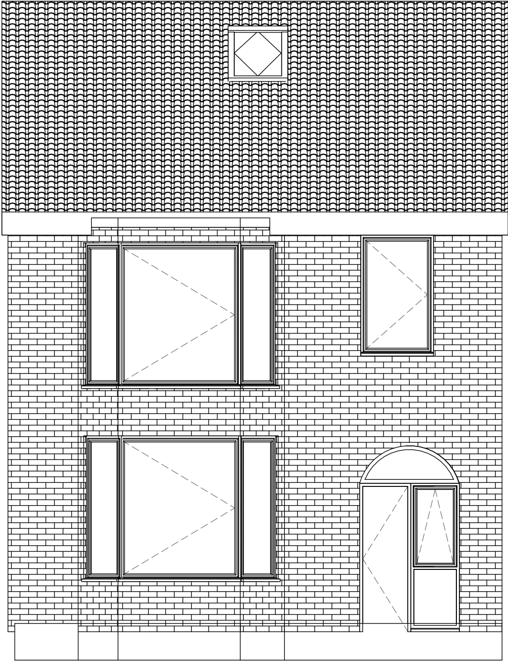
South-West Elevation 1 : 50
