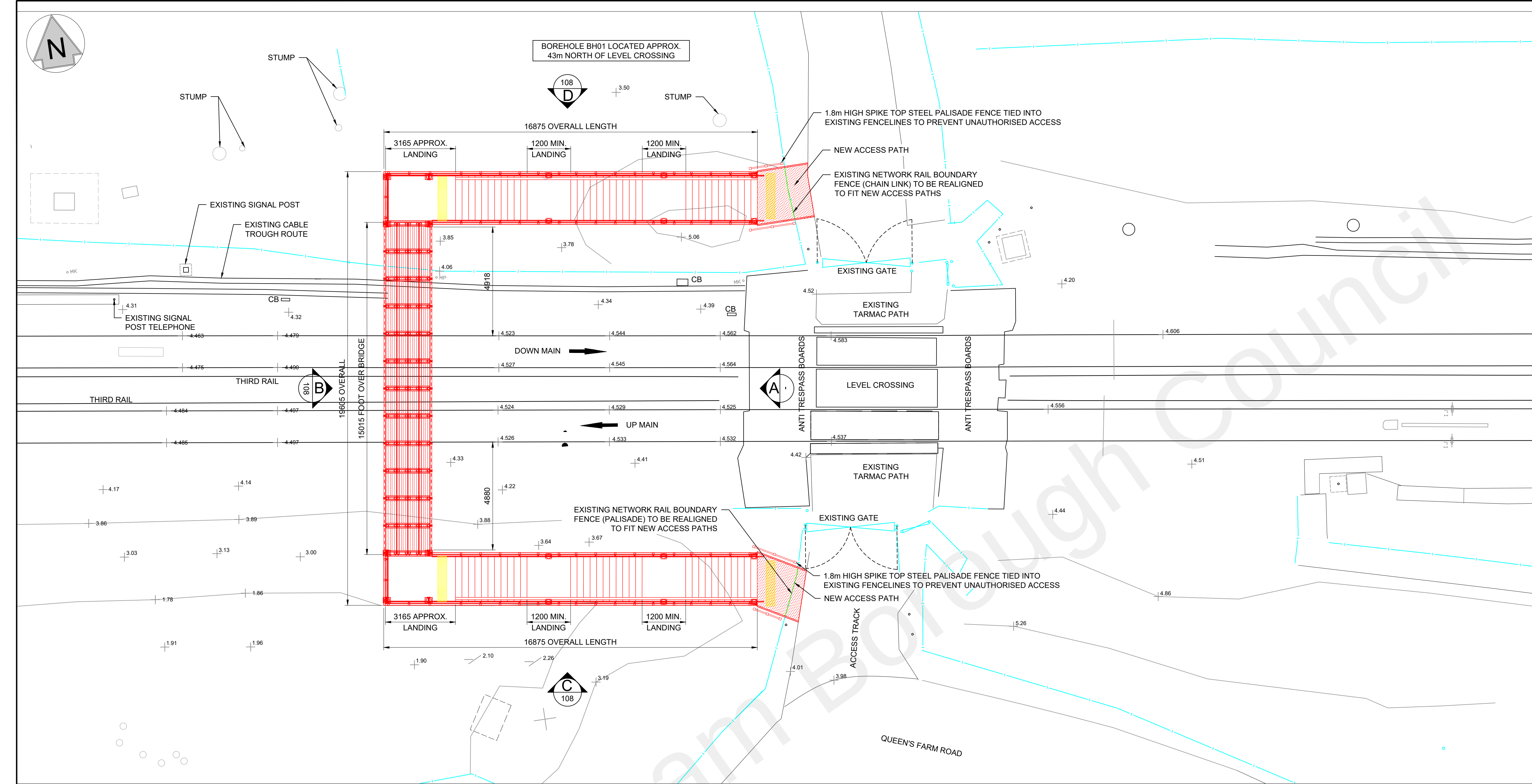
LAYOUT PLAN SCALE 1:100
