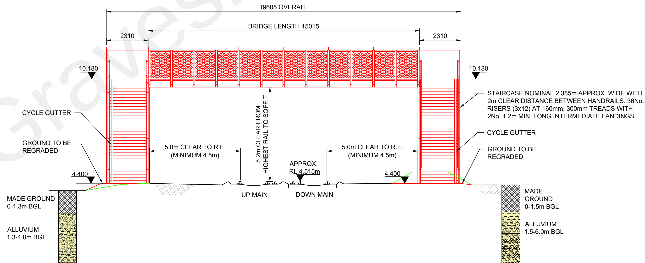
ELEVATION AT A STAIRCASES SHOWN INDICATIVELY SCALE 1:100
