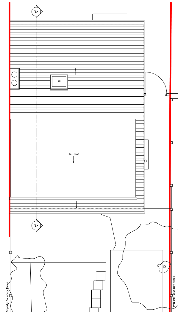
roof plan 1:100
