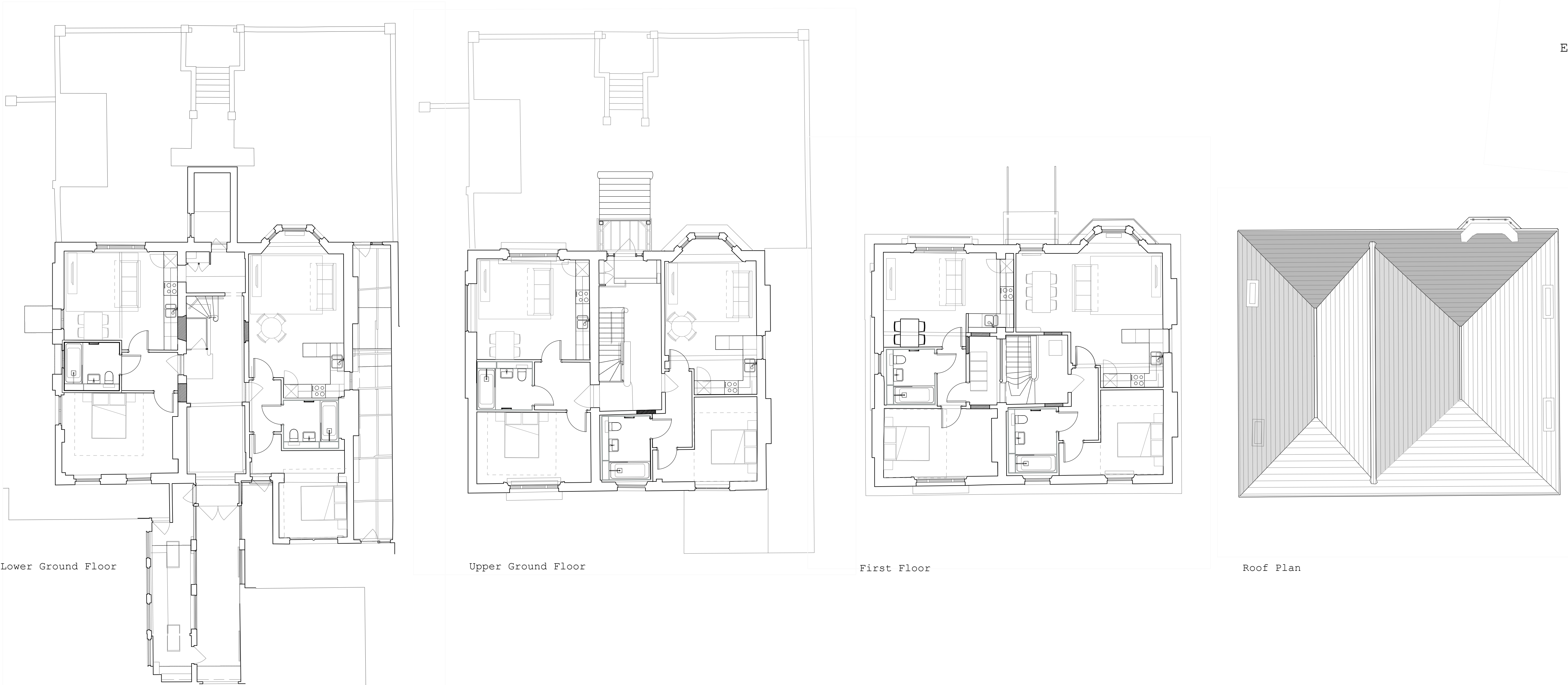
Proposed Plans @1:100
