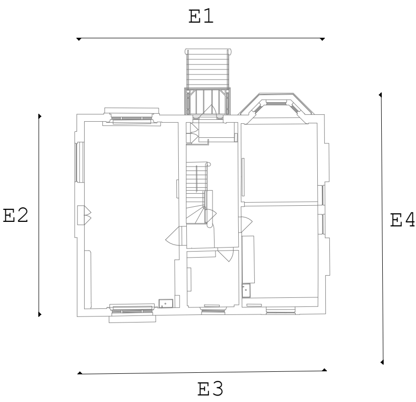
Key Plan @1:200
