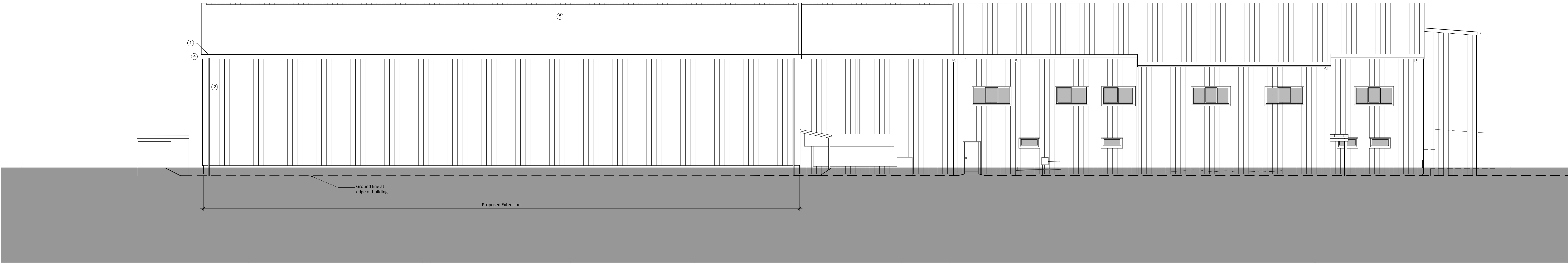
Proposed East Elevation 1:100
