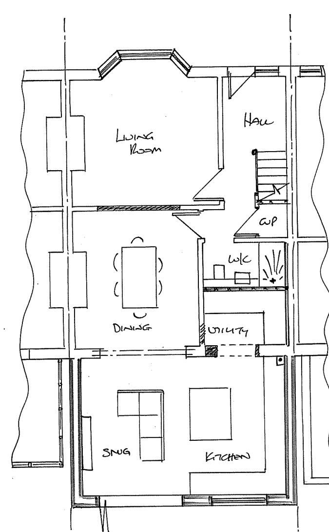
Proposed Ground Floor GA
