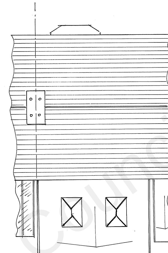
Proposed Roof GA
