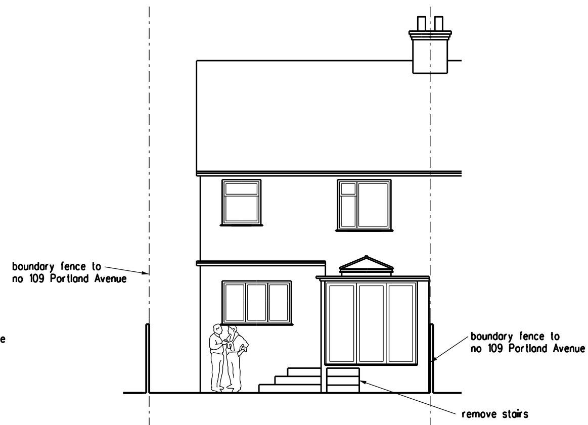
REAR ELEVATION
