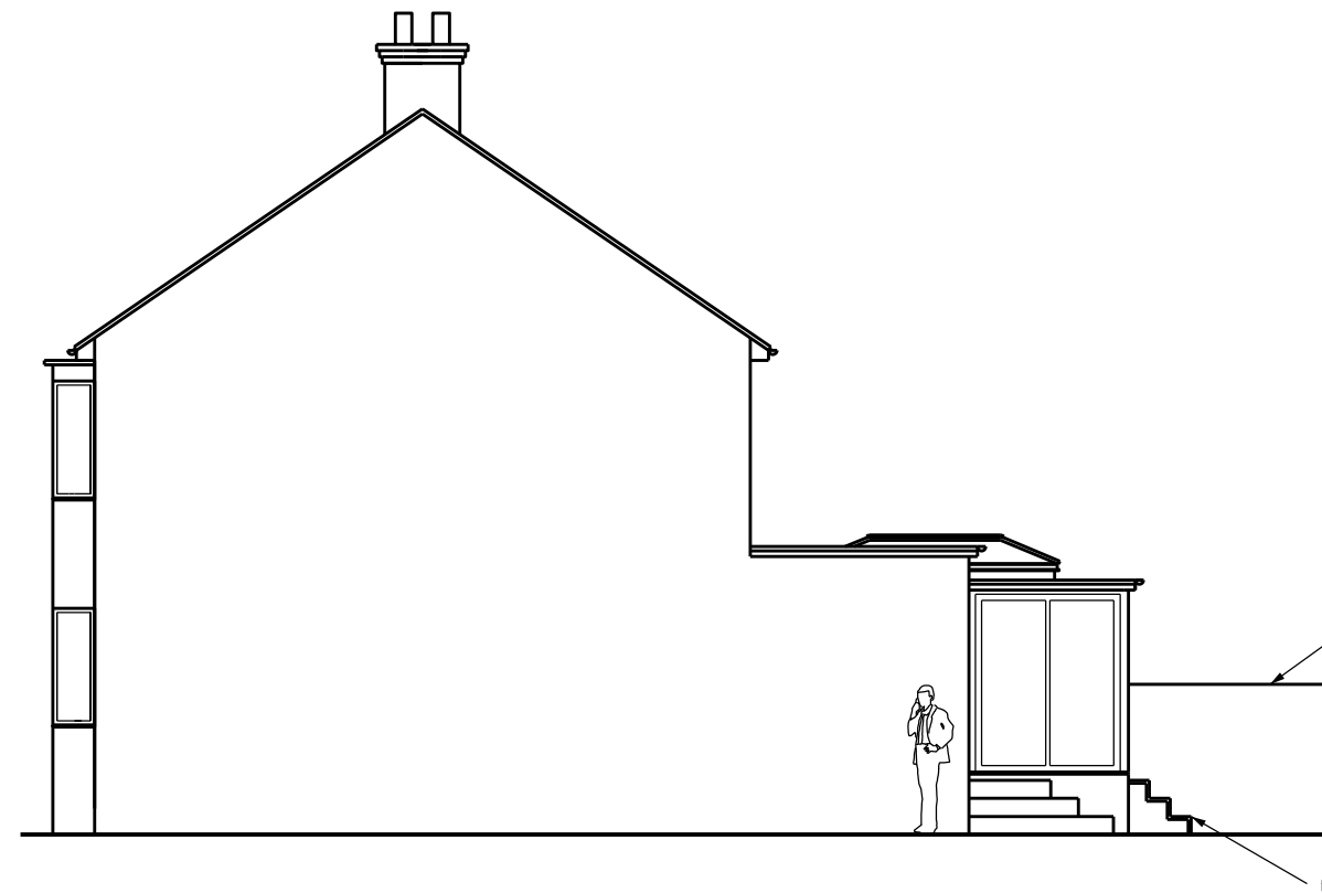
SIDE ELEVATION FACING No 108 PORTLAND AVENUE
