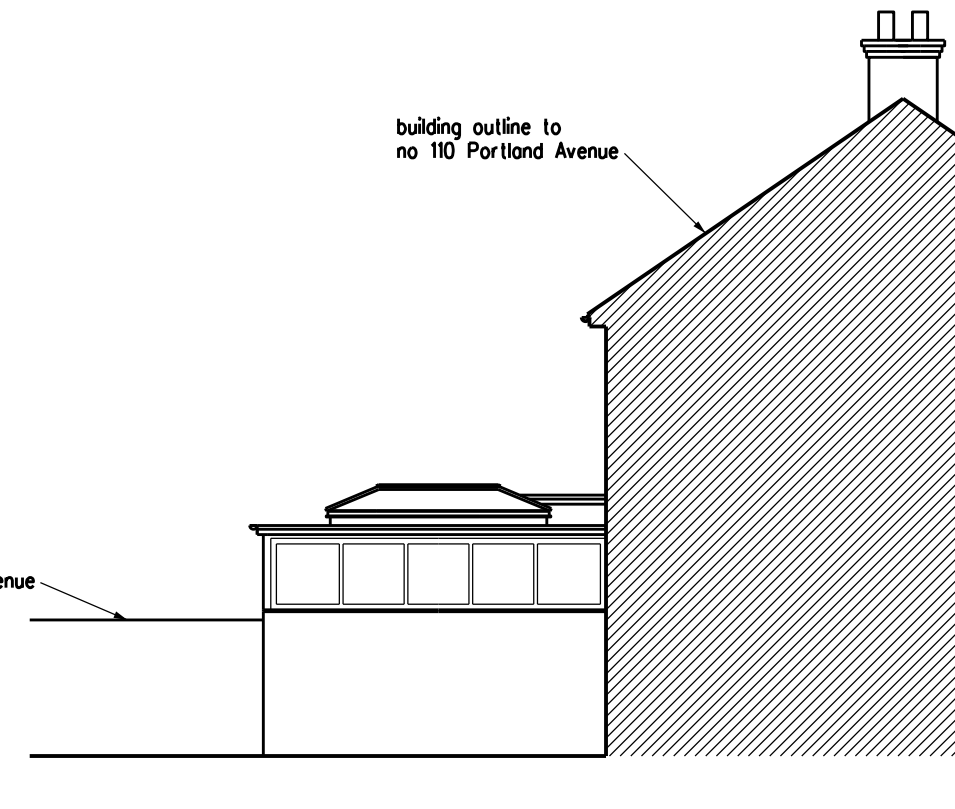
SIDE ELEVATION FACING No 110 PORTLAND AVENUE
