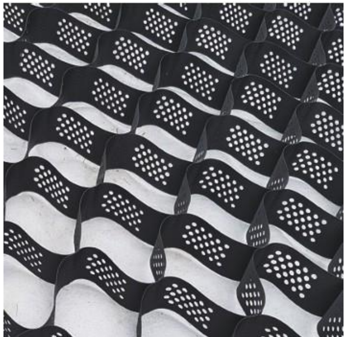
Figure 2- An expanded geocellsh before it has been filled with stone (image courtesy of Bosky Trees)
