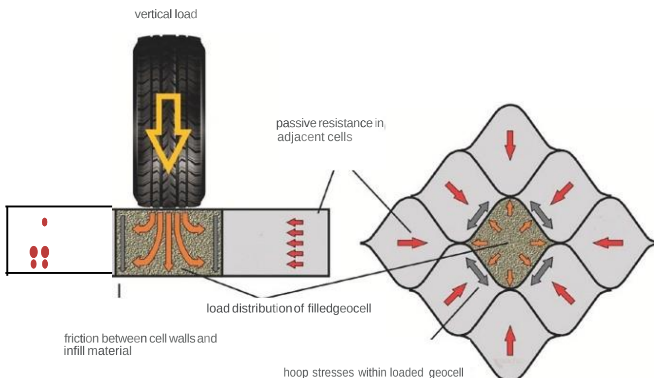
Figure 3: The diagram illustrates the forces and stress distribution when a vertical load is applied to a cellular confinement system (image courtesy of Professor Geosynesis [Greenix])
