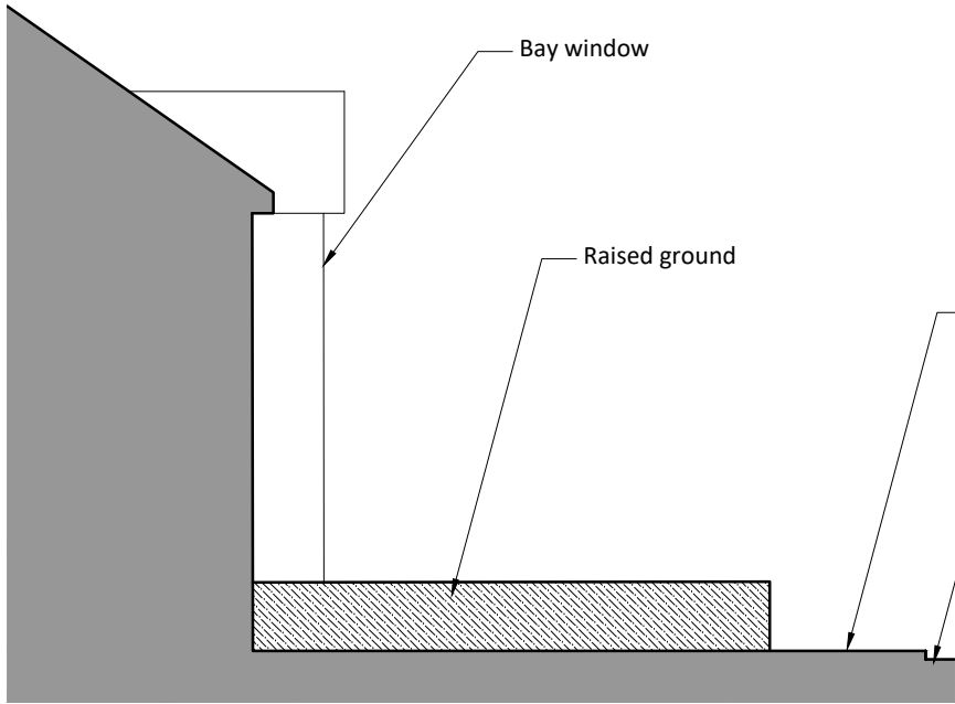
Existing Side (East) Section A 1:100
