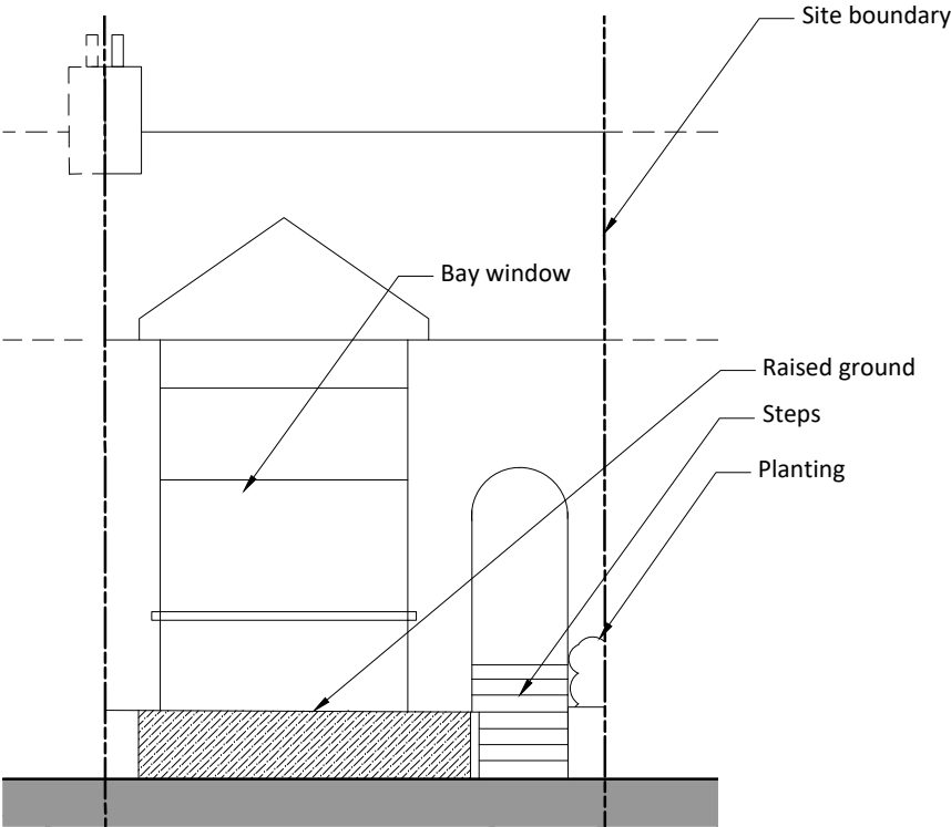
Existing Front (North) Elevation 1:100
