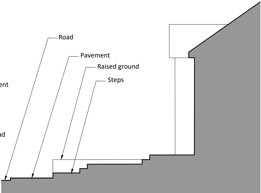
Existing Side (West) Section B 1:100
