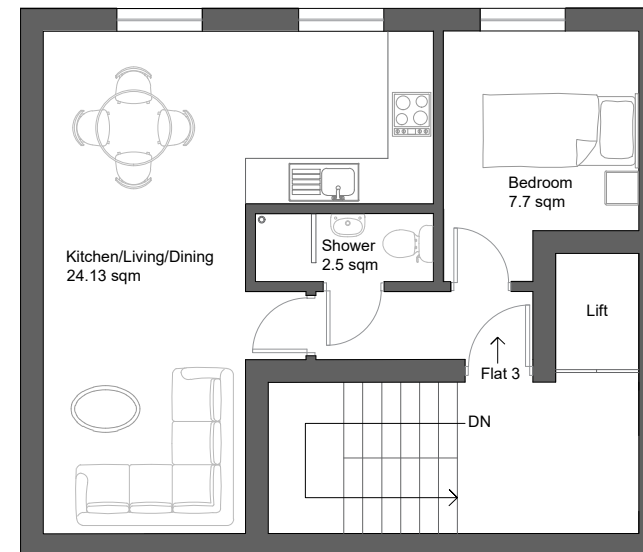
Proposed Third Floor Plan
