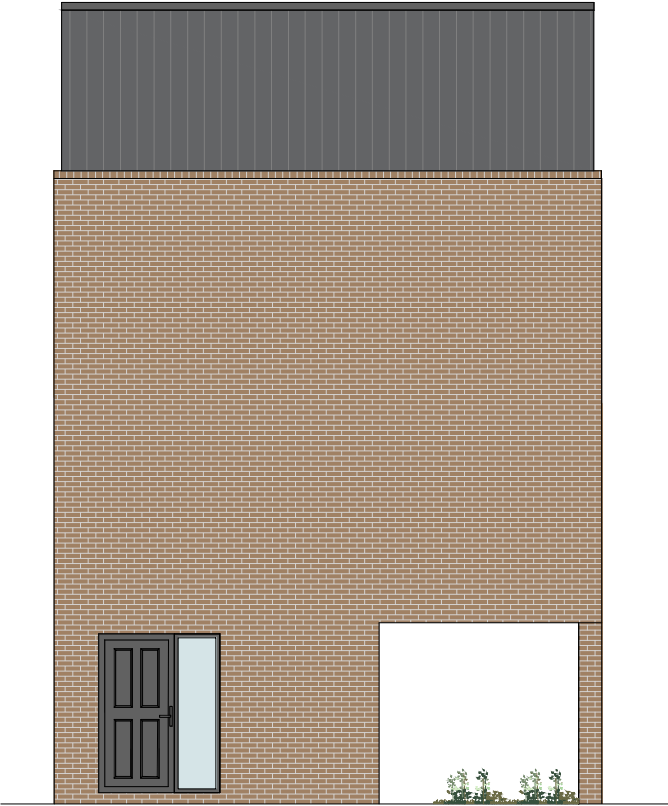
Proposed East Elevation (Side)
