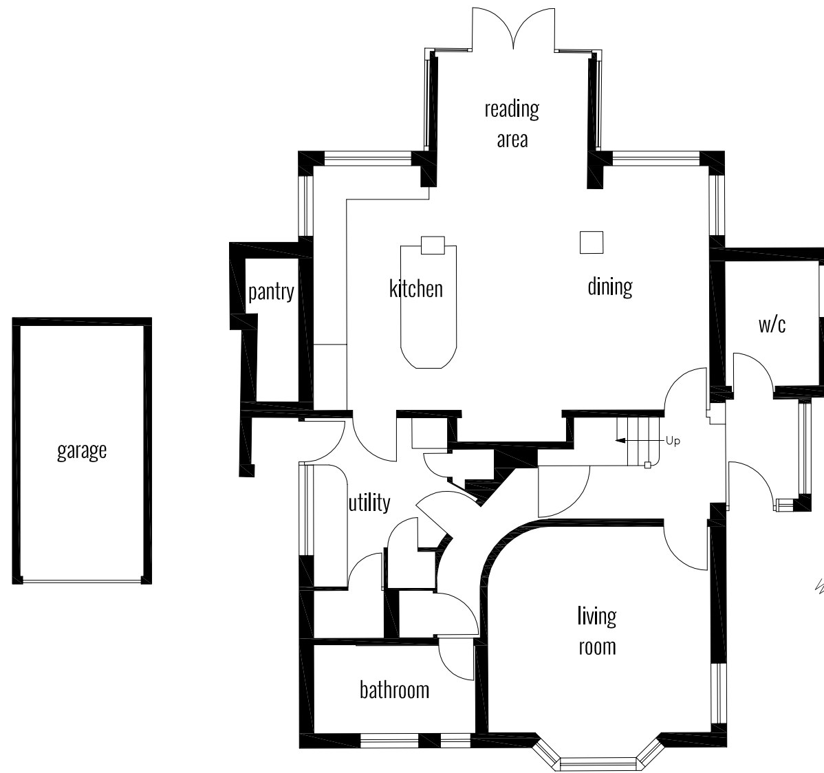
Ground Floor | Existing
