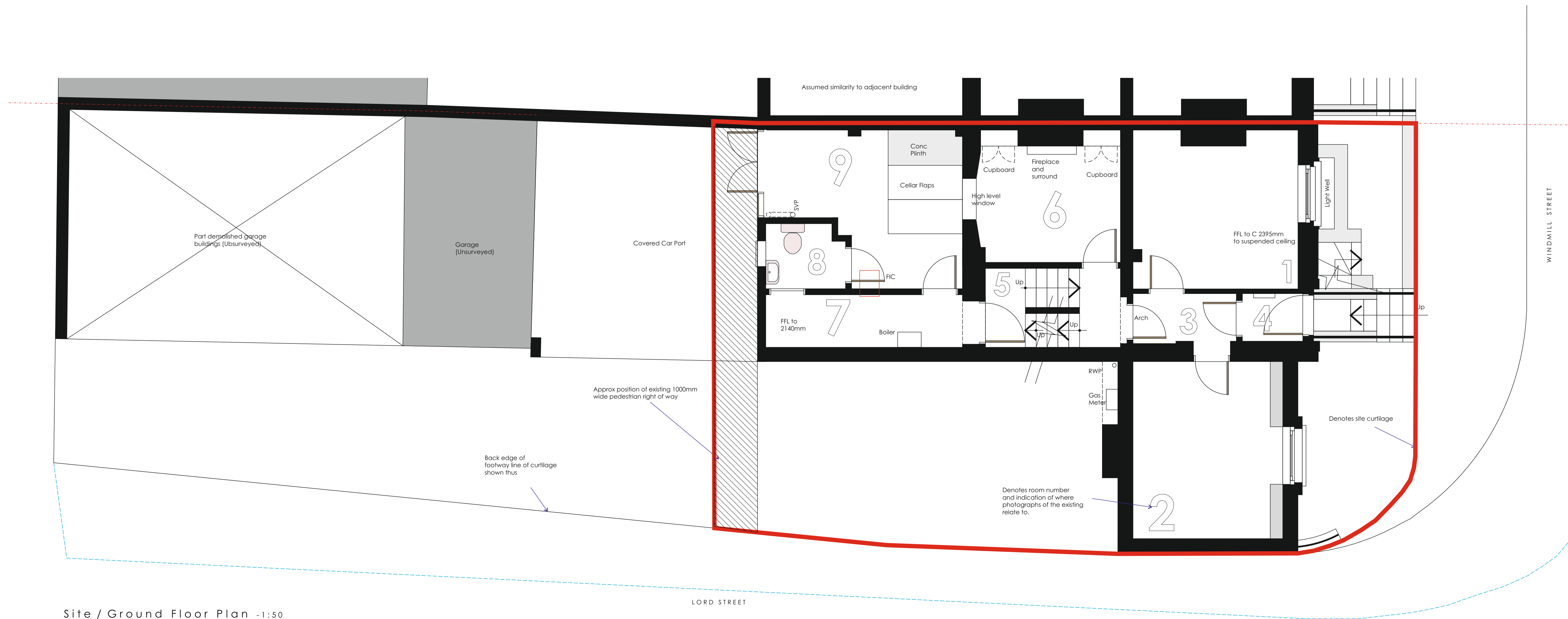
Site / Ground Floor Plan -1:50
