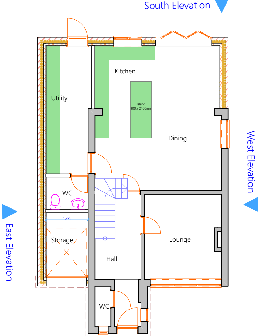
12 GF Ground Floor Proposed 1:100
