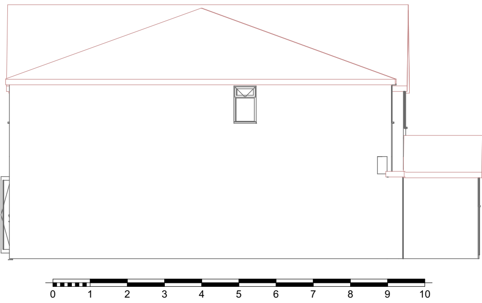
8 East Elevation Proposed 1:100
