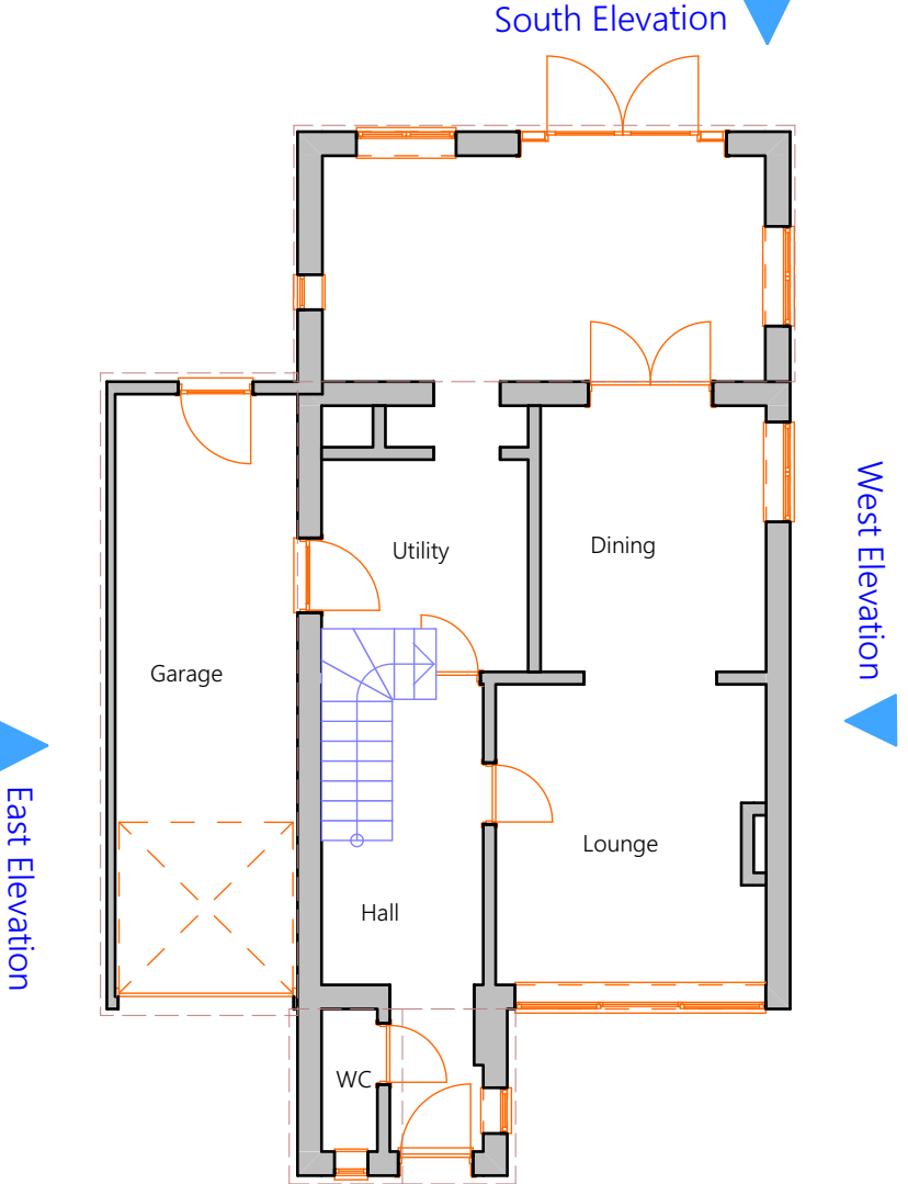
5 GF Ground Floor Existing 1:100
