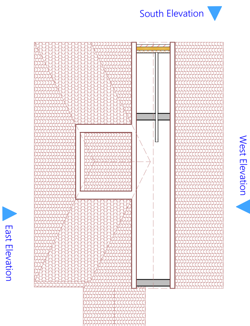
14 Roof Proposed 1:100
