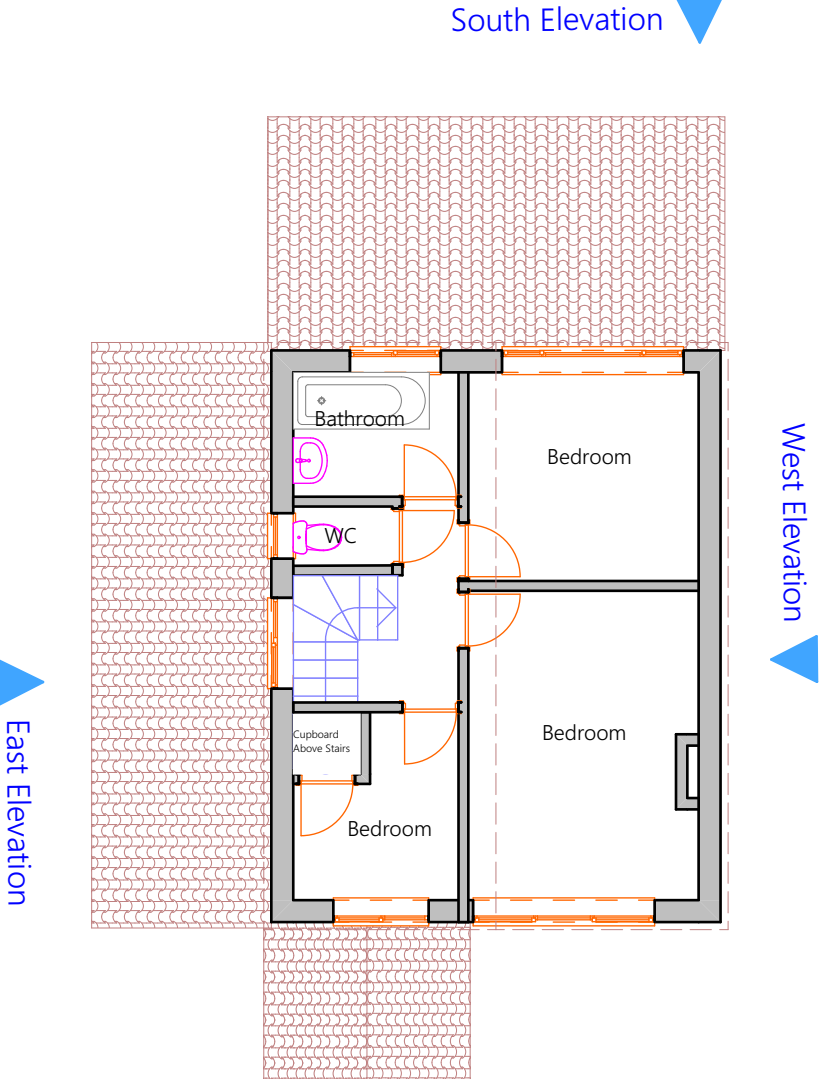
6 01 First Floor Existing 1:100
