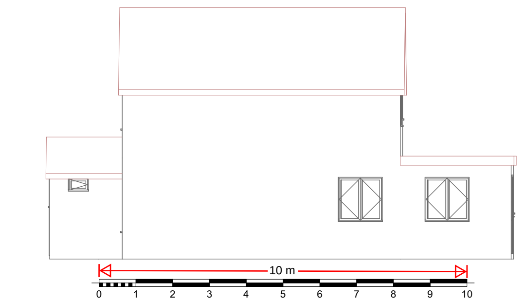
2 West Elevation Existing 1:100
