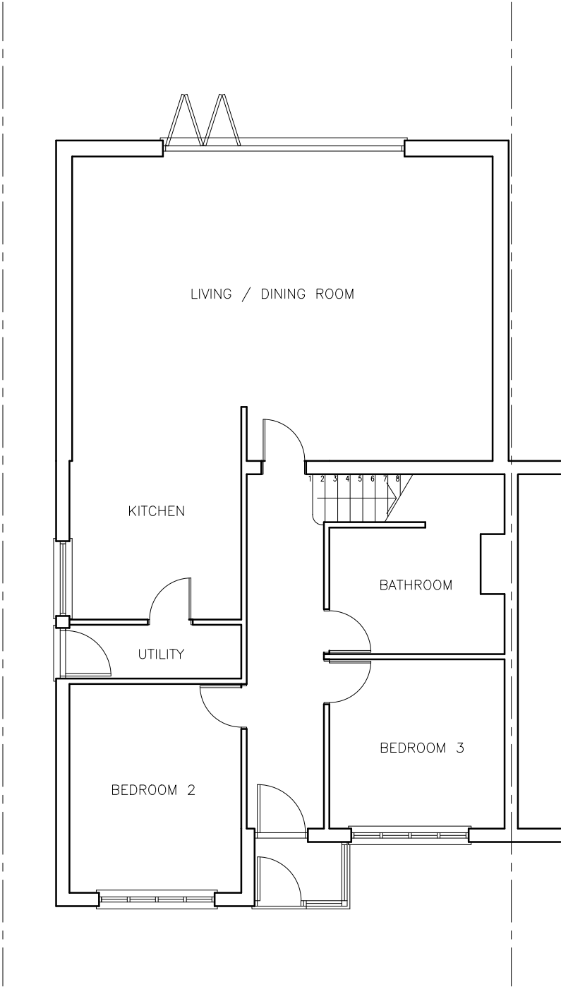
GROUND FLOOR PLAN AS PROPOSED
