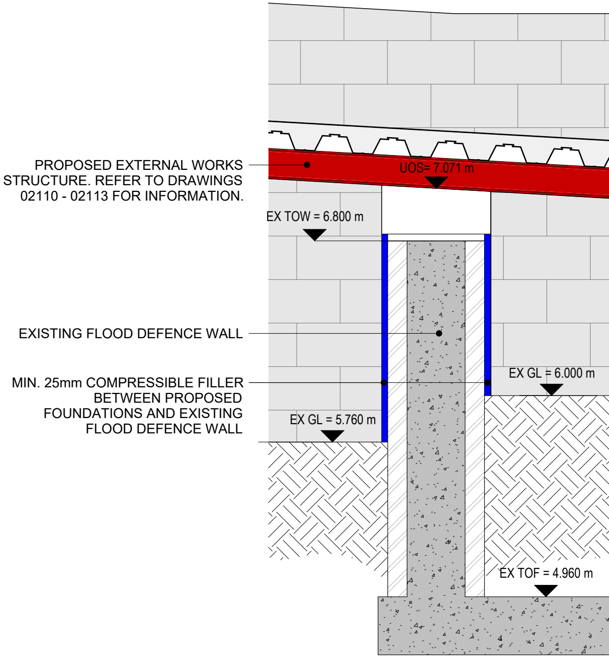
G EXTERNAL WORKS SECTION G 1 : 20
