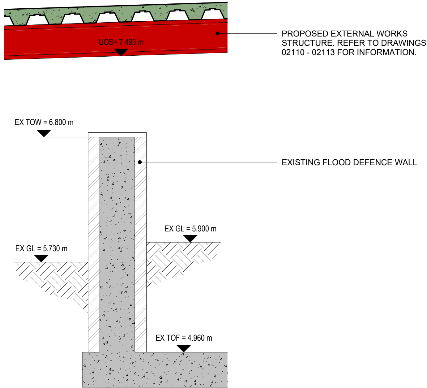
H EXTERNAL WORKS SECTION H 1 : 20
