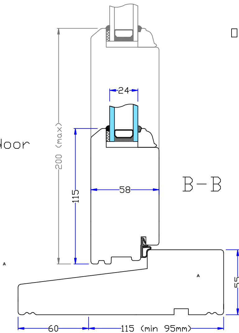
60mm extended hardwood sill
