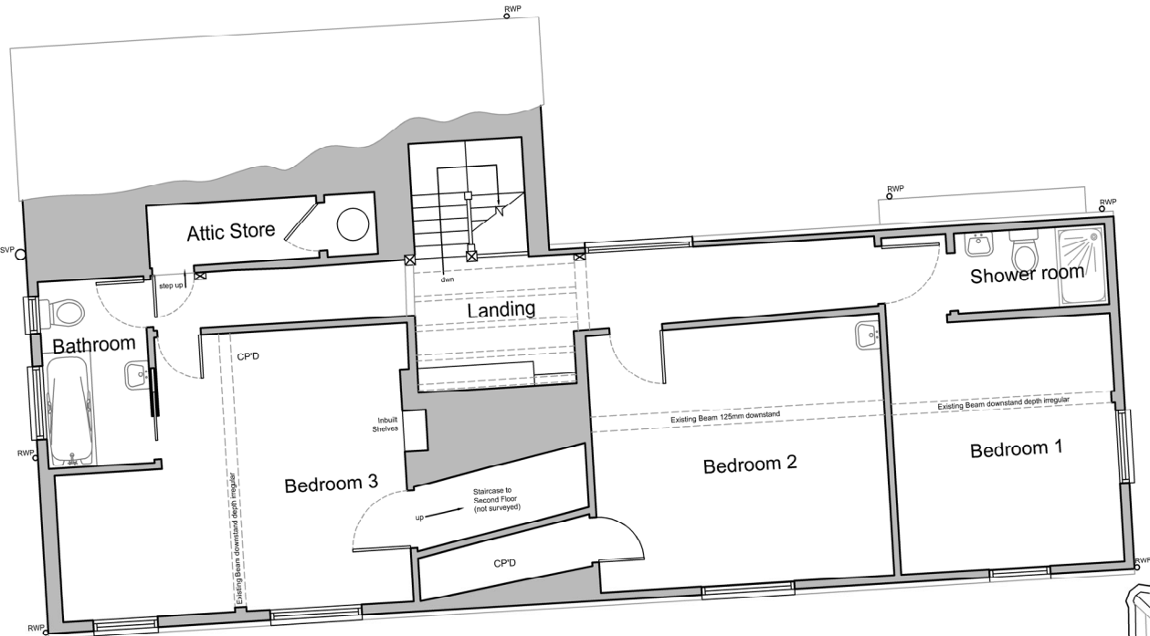
Proposed First Floor Plan Scale 1:100 @ A3
