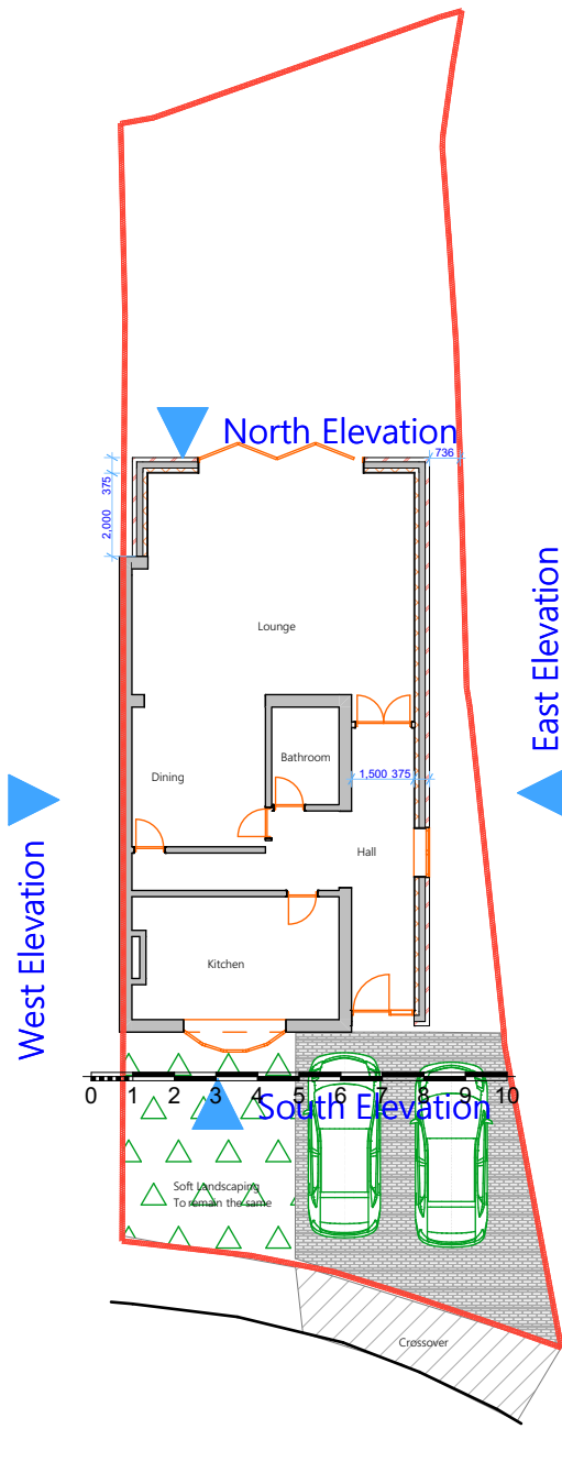
3 Site Plan Proposed 1:200
