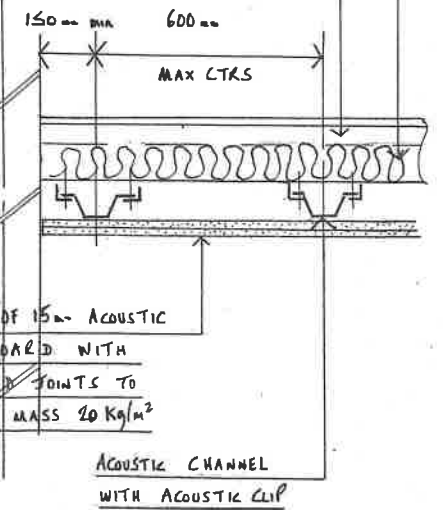
DETAIL A 1:10 AT A1 HORIZONTAL SOUNDPROOFING
