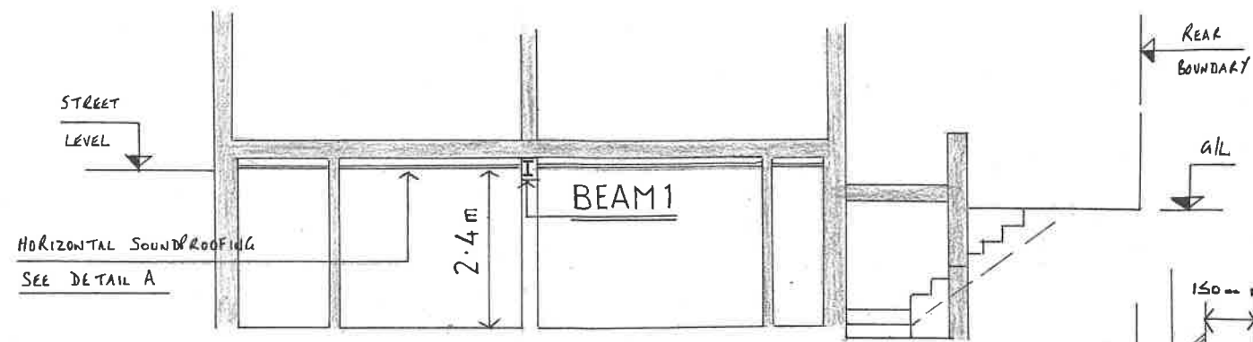
SECTION 1-1
