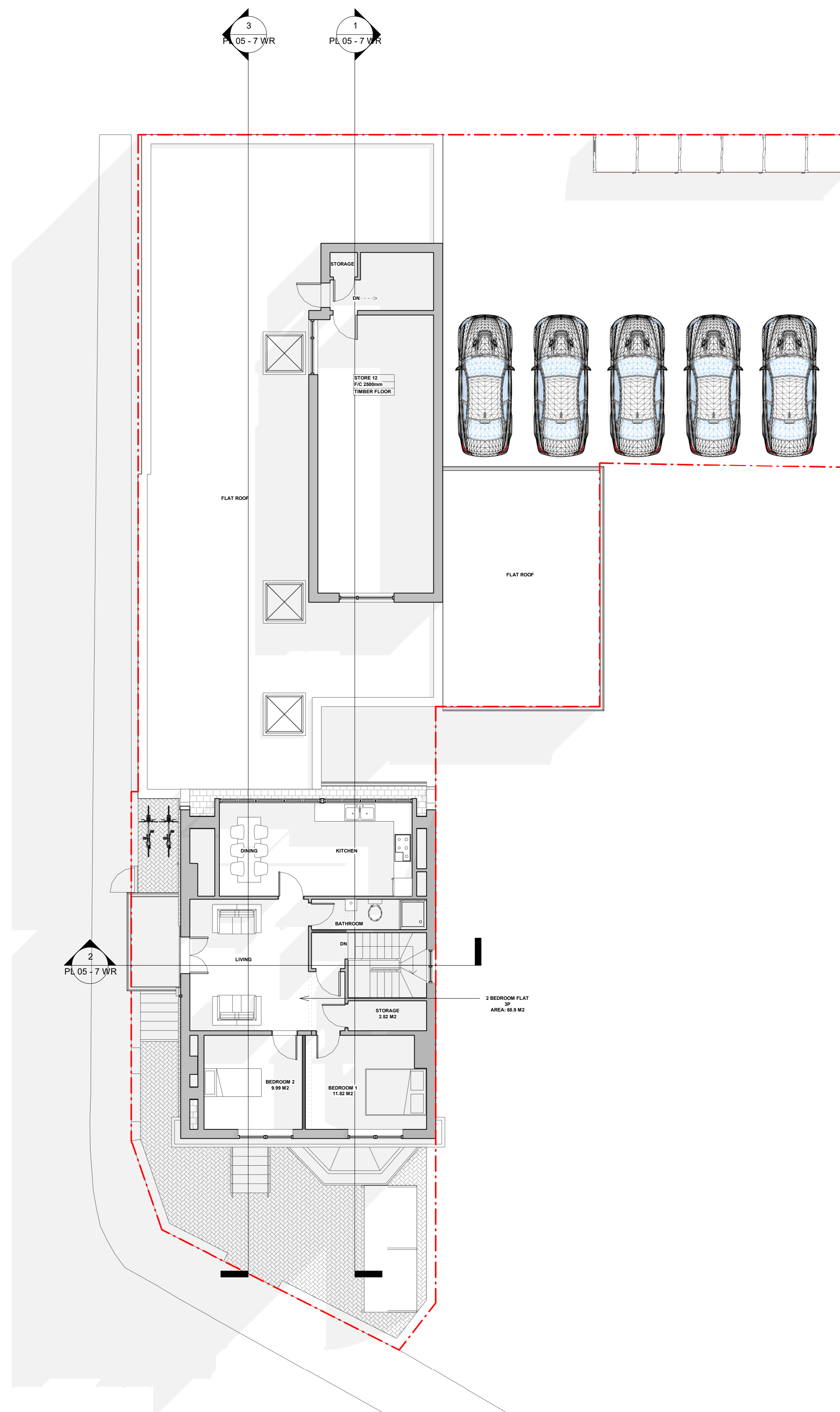
2 Approved Loft 1 : 100
