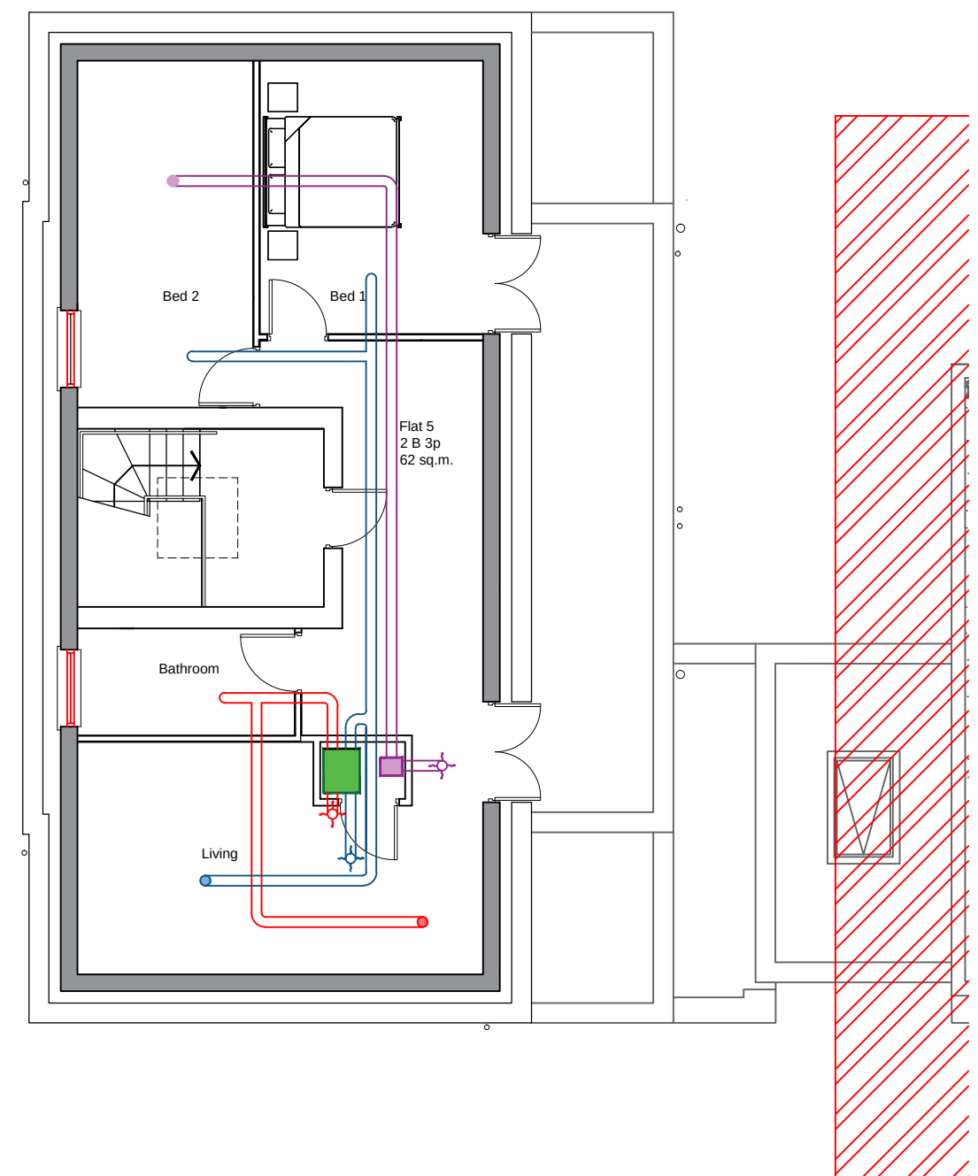
Second Floor
